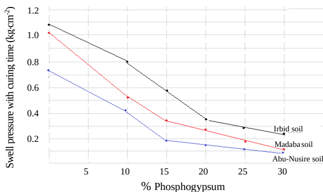
Figure 12. Swell pressure vs percent admixture of phosphogypsum at zero day curing time for Irbid, Madaba and Abu-Nusire soils.
