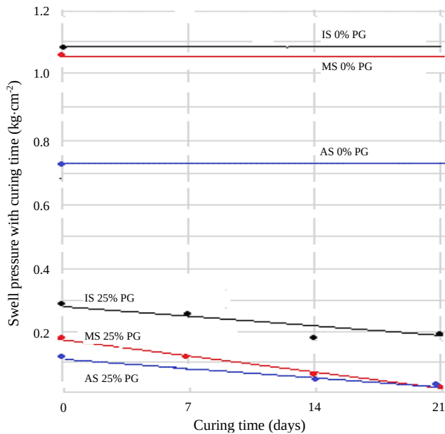
Figure 14. Variation of swell pressure with curing time for untreated and treated Irbid, Madaba and Abu-Nusire soils with different phosphogypsum contents.
