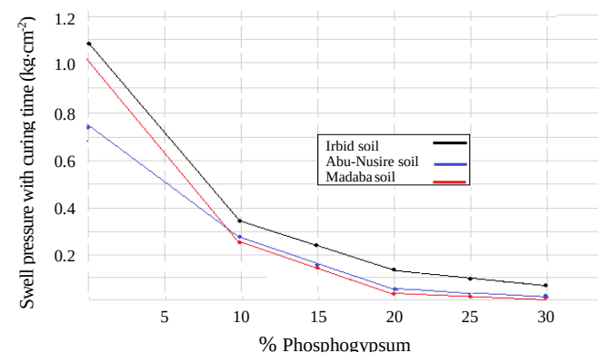
Figure 13. Swell pressure vs. percent admixture of phosphogypsum at 21 days curing time for Irbid, Madaba and Abu-Nusire soils
