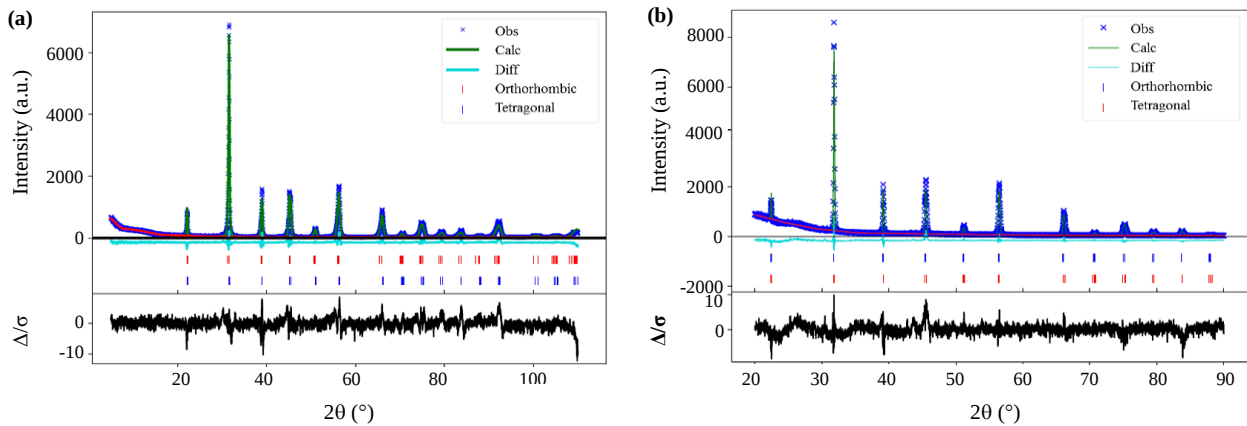
Figure 5. The observed, calculated and difference curves obtained by Rietveld refinement for (a) BCZT powder and (b) BCZT ceramic, showing the best fit with the coexistence of orthorhombic and tetragonal.
