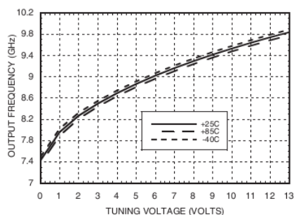
Frequency vs. Tuning Voltage, V_{CC} = +5V
