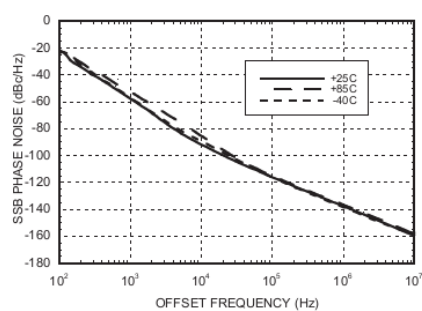
SSB Phase Noise @ V_{tune} = +5V
