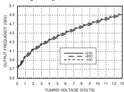
RFOUT/2 Frequency vs. Tuning Voltage, Vcc = +5V
