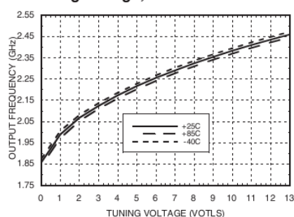
Divide-by-4 Frequency vs. Tuning Voltage, Vcc = +5V
