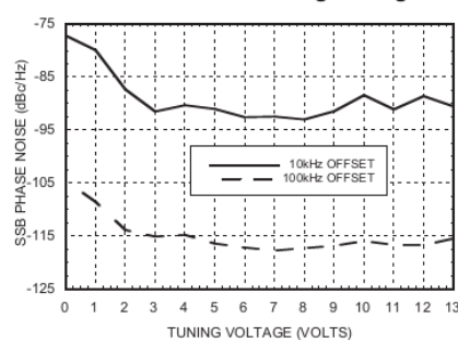
SSB Phase Noise vs. Tuning Voltage
