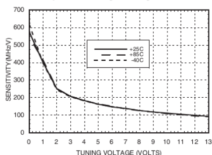
Sensitivity vs. Tuning Voltage, V_{CC} = +5V
