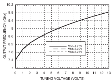
Frequency vs. Tuning Voltage, T = 25^{\circ}C
