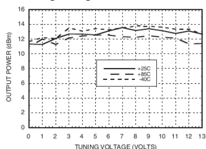
Output Power vs. Tuning Voltage, V_{CC} = +5V
