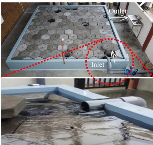
Fig. 1. Field test of multi-chamber stormwater detention system.
