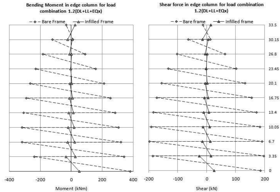
Figure 32 Comparison force in edge column for full infill
