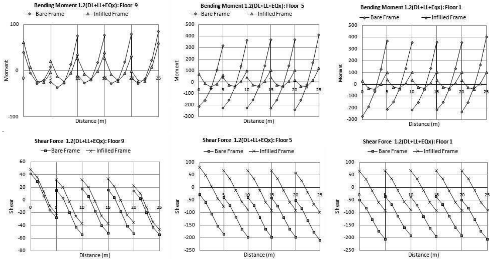
Figure 39 Member forces in edge beam for full infill
