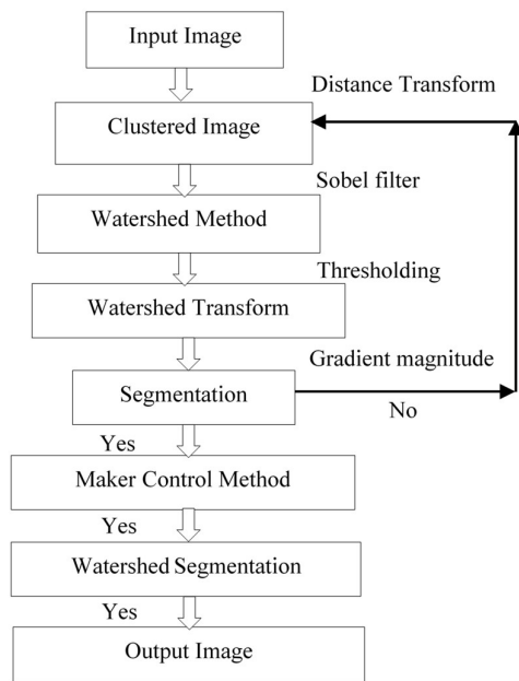
Figure 2 Algorithm watershed Segmentation
