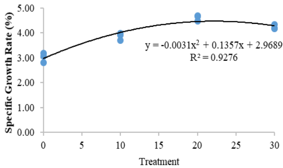
Figure 1. Polynomial Orthogonal Graph and Curve Analysis Result for Specific Growth Rate (SGR)
