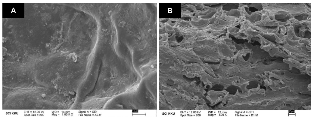
Fig. 3. Scanning electron microscopic (SEM) image of untreated MLW (A) and hydrolyzed MLW by cellulase, after pretreatment with 1% (v/v) \text{H}_2\text{SO}_4 at 121^\circ\text{C} for 90 min (B).
