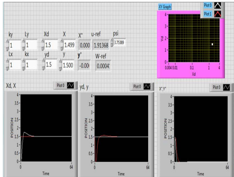
Figure 5: Kinematic control.
