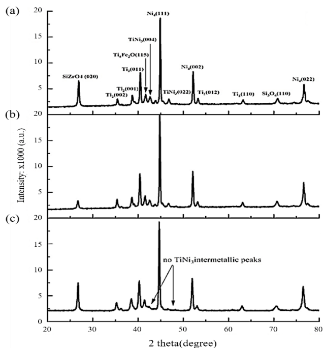
Figure 6. Representative XRD spectra for samples (a) CCS-T1, (b) CCS-T2 and (c) CCS-T3.
