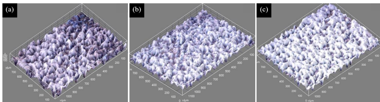
Figure 7. 3-D surface morphology of the MMCs (a) CCS-T1, (b) CCS-T2 and (c) CCS-T3.
