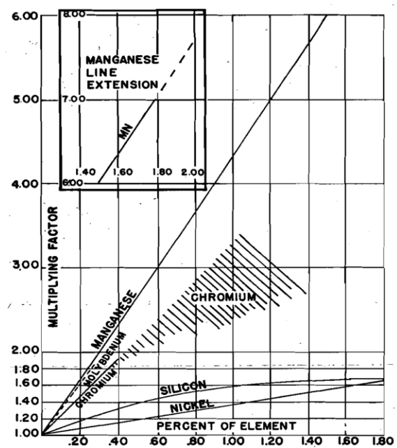
Figure 4. Hardenability multiplying factors for common alloying elements [38] (with permission from AIST).
