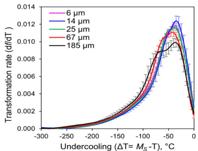
Figure 5. Martensite transformation rate ( df/dT ) against undercooling ( \Delta T ). The transformation starts at zero undercooling, which corresponds to the M_s at which the fraction of formed martensite is f_{\alpha'} = 0.01 [41].
