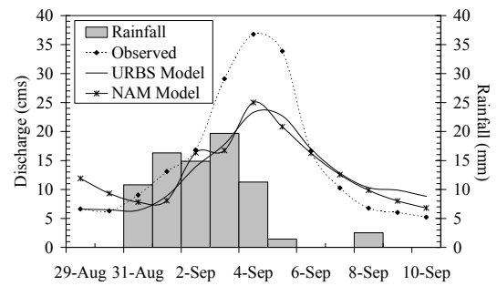
b) Flood hydrograph in 1996
