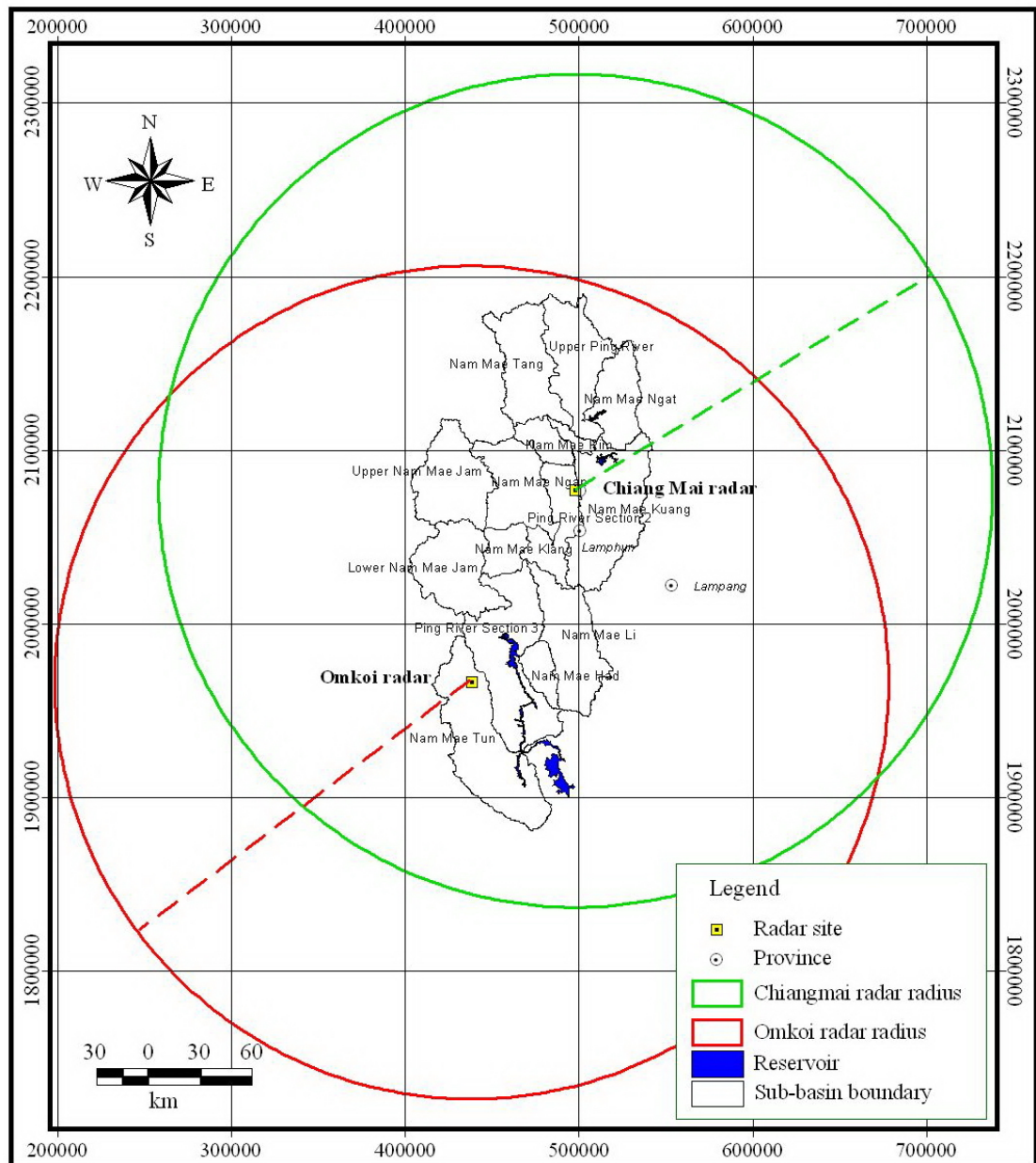
Figure 13 Location of weather radar belonged to the BRRAA and the TMD covering the upper Ping river basin.
