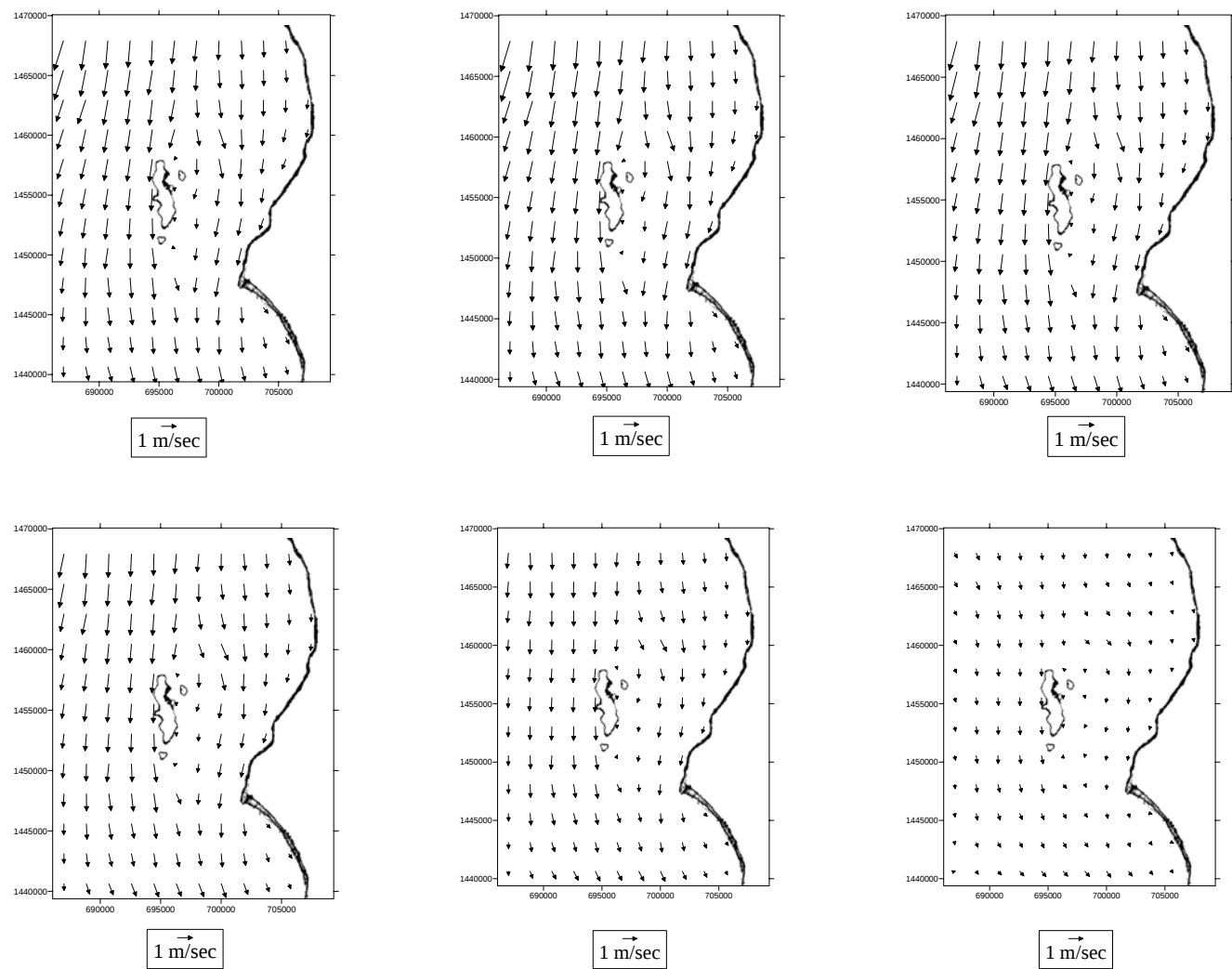
Figure 21 Distribution patterns of tidal stream 24 hours in Ao Si Racha
