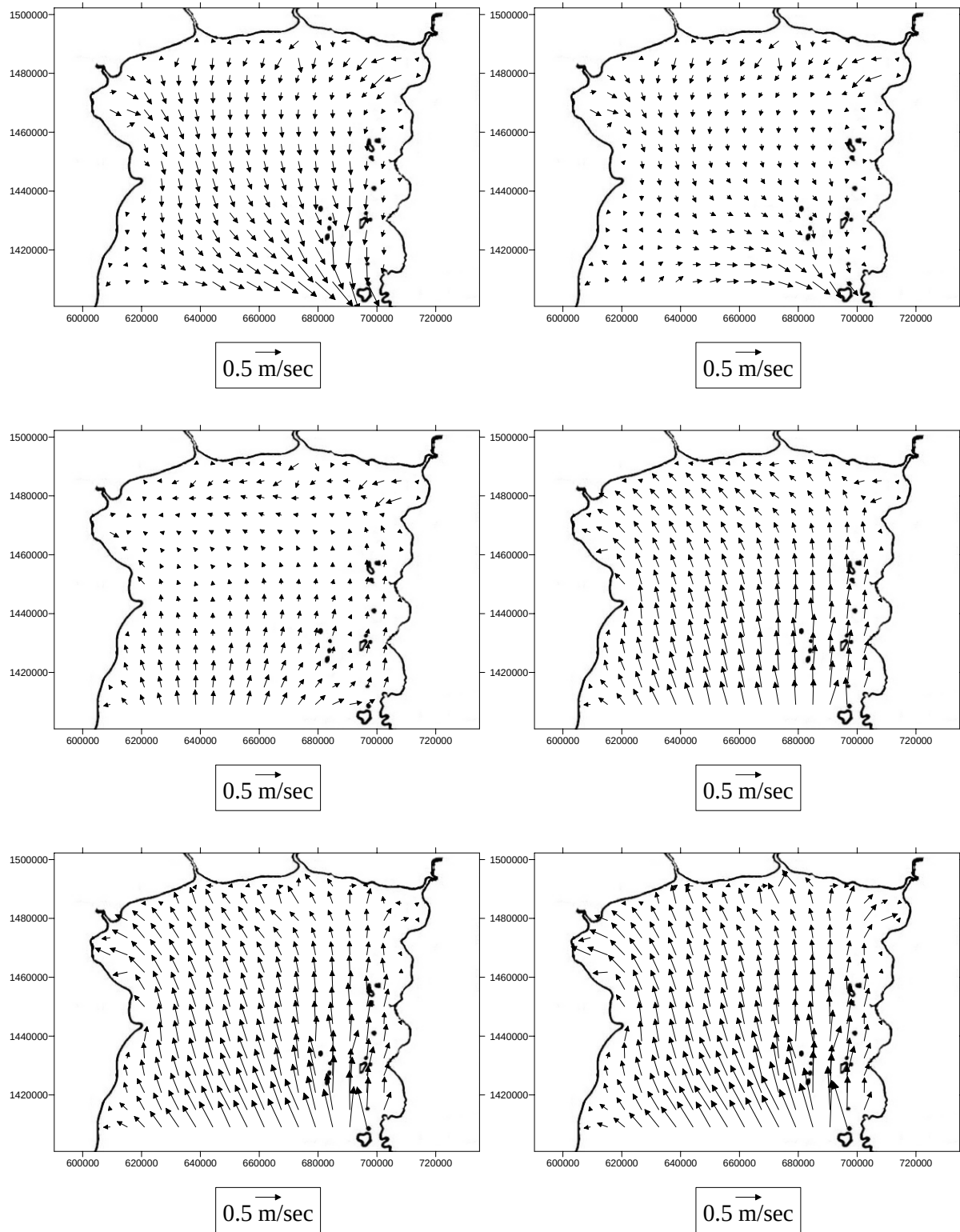
Figure 20 Distribution patterns of tidal stream 24 hours in the upper Gulf of Thailand
