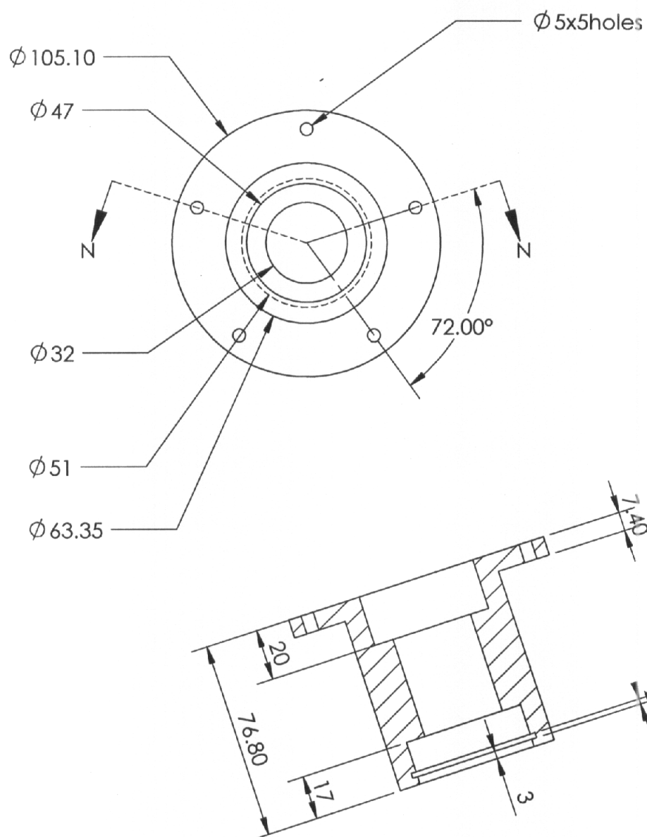
SECTION N-N
