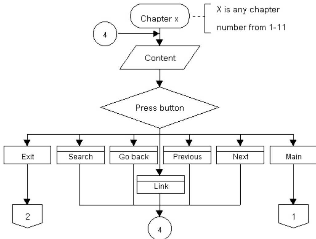
Figure I.10 Flowchart in module “Chapter X”
