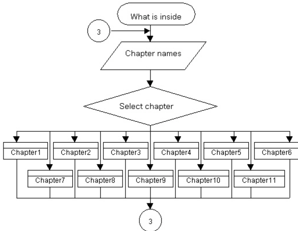
Figure I.9 Flowchart in module “What is inside”
