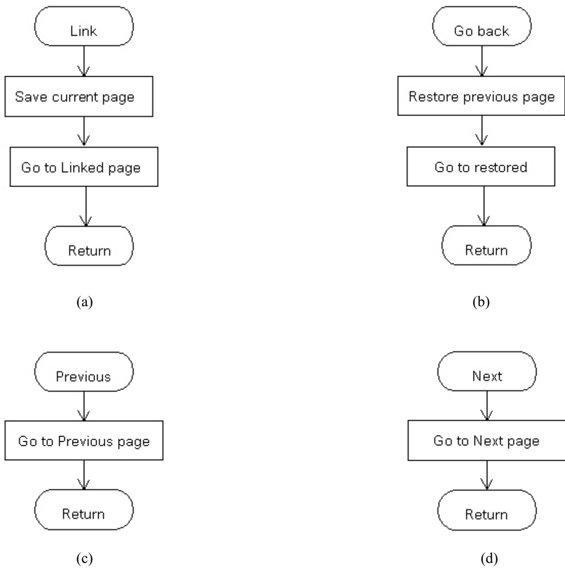
Figure I.11 Flowchart in module of button : (a) Link, (b) Go back, (c) Previous, (d) Next.
