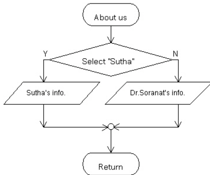
Figure I.7 Flowchart in module “About US”
