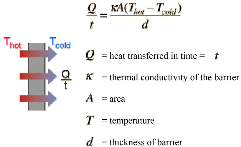
Figure 2-5 Heat conduction transfer rate
