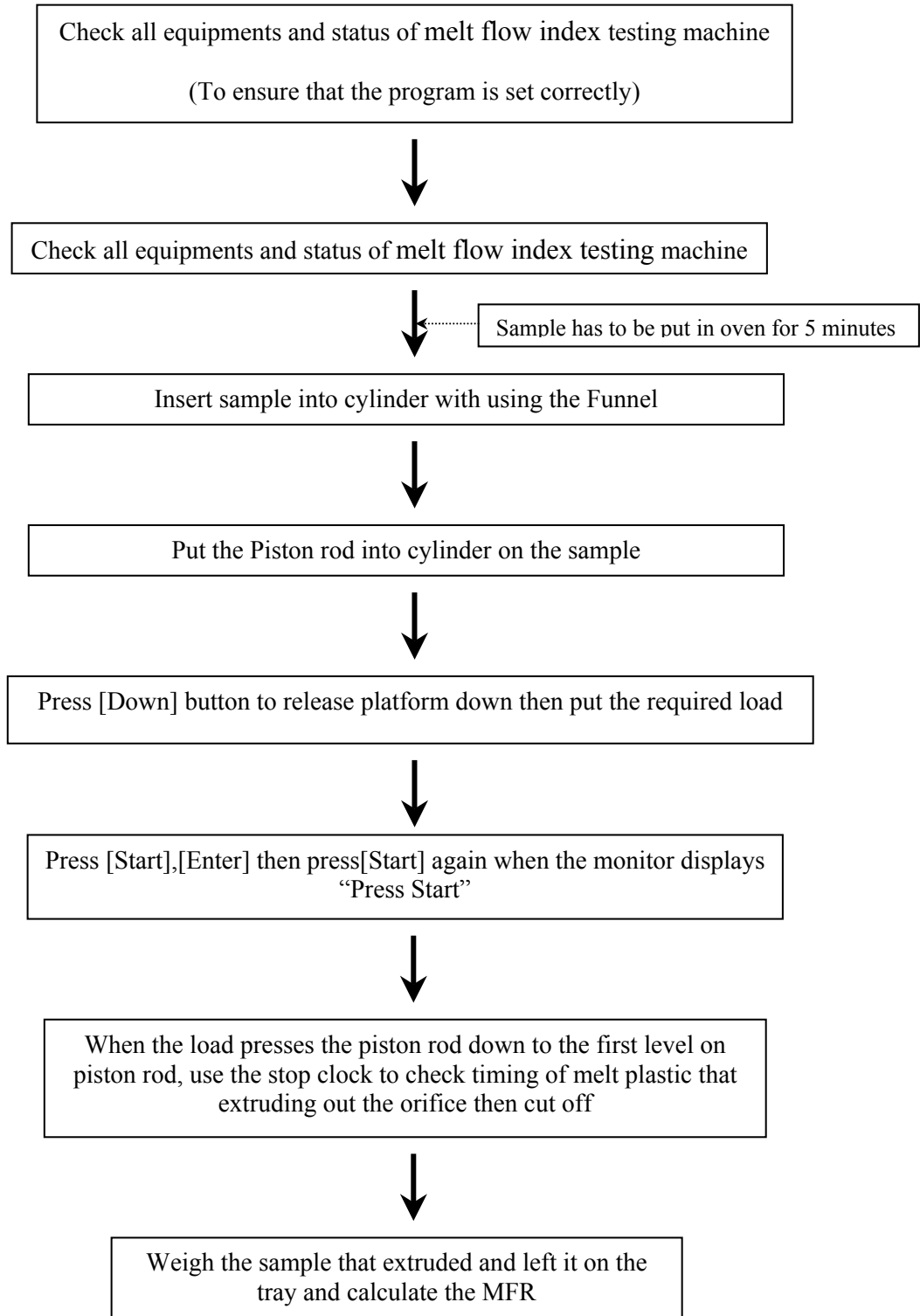
Figure 2-2 Melt flow testing steps
