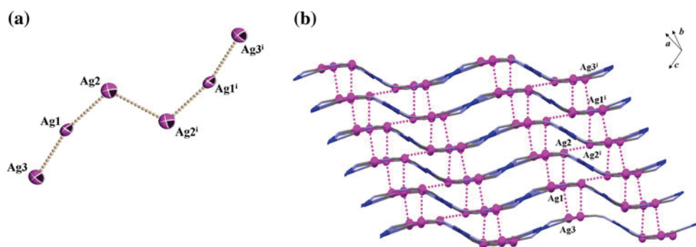
Fig. 2 a Hexanuclear \text{Ag}^{\text{I}} unit (symmetry code i = 1-x, 1-y, -z ), b side view of multiple-layer 3D network via hexanuclear \text{Ag}^{\text{I}}\cdots\text{Ag}^{\text{I}} interactions Hydrogen atoms, coordinated ampyz, water and lattice ampyz molecules are omitted for clarity
