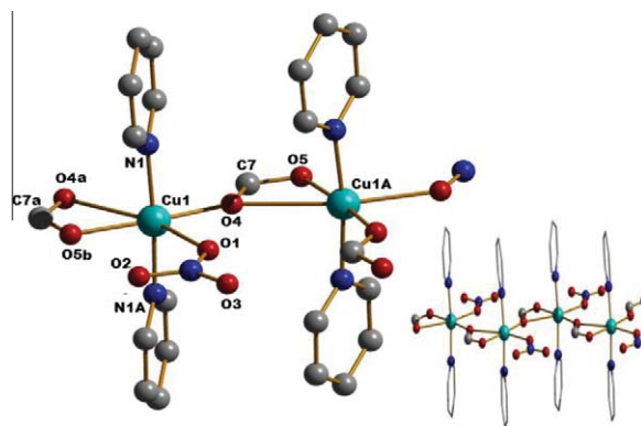
Fig. 4. Left: representation of the dinuclear unit of 2 with the atom-labelling scheme. Right: formation of a 1D chain through formate bridges.
