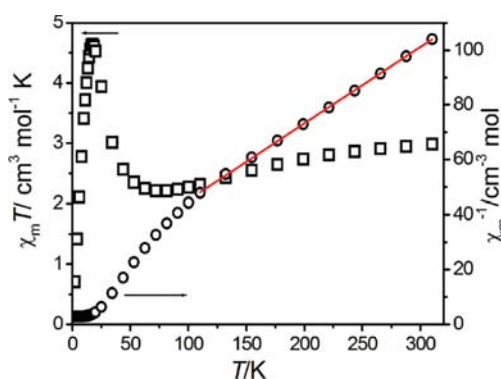
Figure 5. Temperature dependence of \chi_m T (□) and \chi_m^{-1} (○) of 1 from 2 to 310 K at H = 10 kOe. The solid lines correspond to the best fit to the Curie–Weiss law.
