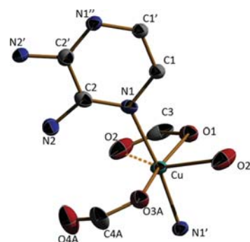
Figure 1. Asymmetric unit and atom labeling scheme of 1 . The ellipsoids are shown at 35% probability level, and the disordered O3B, C4B, O4B and hydrogen atoms are omitted for clarity. Both disordered positions of N2 are shown. The dashed line represents weak interaction in the off-the-axis position.
