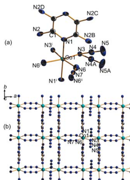
Figure 1. (a) Crystal structure and atom labeling scheme of 1 , (i) x , −y , 2− z ; (ii) −x , −y , z . The ellipsoids are shown at 50% probability level. All disordered positions of amino group and N atoms of EO-azide are shown. (b) 2D layer of 1 in the ab plane. All H atoms are omitted for clarity.
