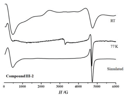
Figure 20 EPR spectra of III-2 at RT and 77 K and the simulation for dinuclear Cu II at 77 K.
