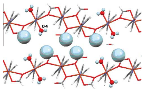
Fig. 3. Illustration of the solid-state structure of 1 showing the absence of steric bulk due to the formate ligands (whose hydrogen atom is shown in the space-filling mode), hence allowing the coordination of two water molecules (O4 and O4b) to the Cu2 centre.
