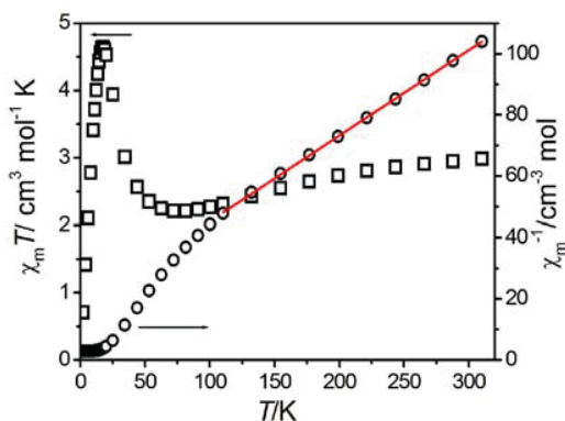
Figure 92 Temperature dependence of \chi_m T (□) and \chi_m^{-1} (○) of V-3 from 2 to 310 K at H = 10 kOe. The solid lines correspond to the best fit to the Curie-Weiss law.
