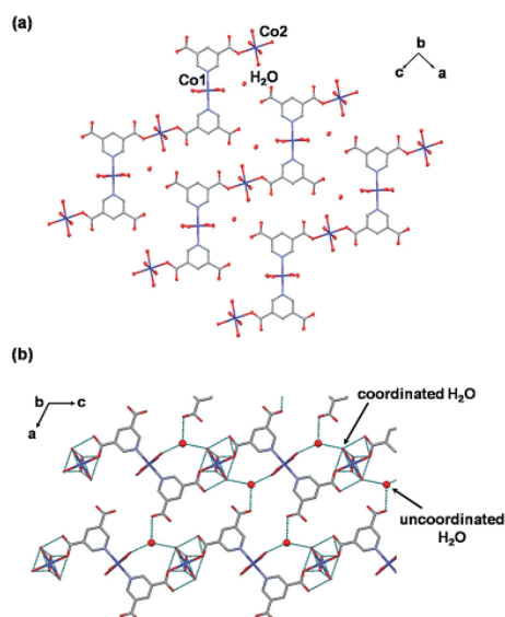
Figure 61 (a) 1D zig-zag chain of IV-6 in the ac plane formed by the \text{Co(II)} and \text{pydc}^{2-} ligand. Water molecule filled in the cavity between chains. (b) The 2D hydrogen-bonded layered network via hydrogen bonds between \text{pydc}^{2-} ligands, coordinated- and uncoordinated water molecules among the 1D zig-zag chains (blue dash lines). All hydrogen atoms are omitted for the clarity.
