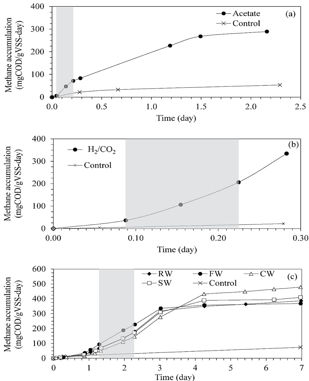
Figure 1 Accumulation of methane over time from (a) acetate, (b) H_2/CO_2 , and (c) the various test wastewater types
