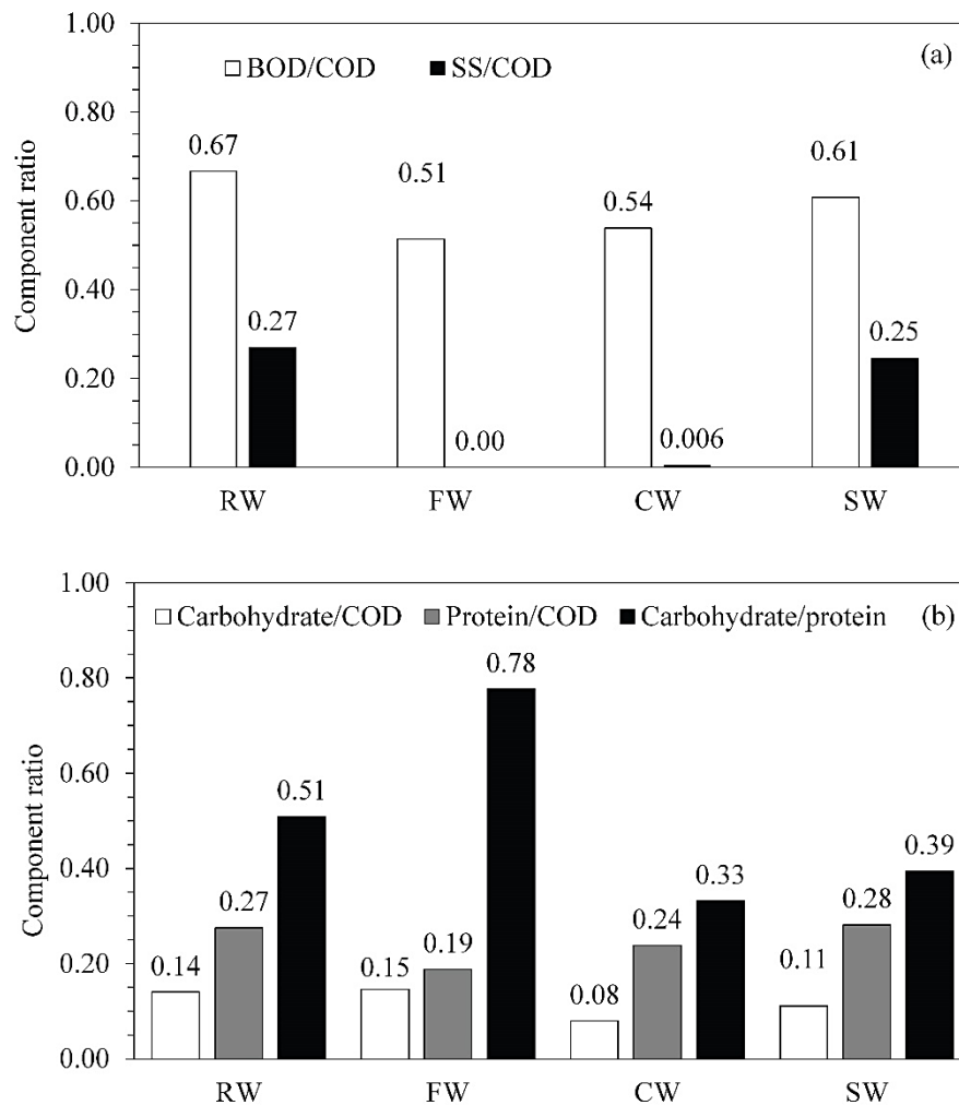
Figure 3 A comparison of the component ratios of the test wastewater types.
