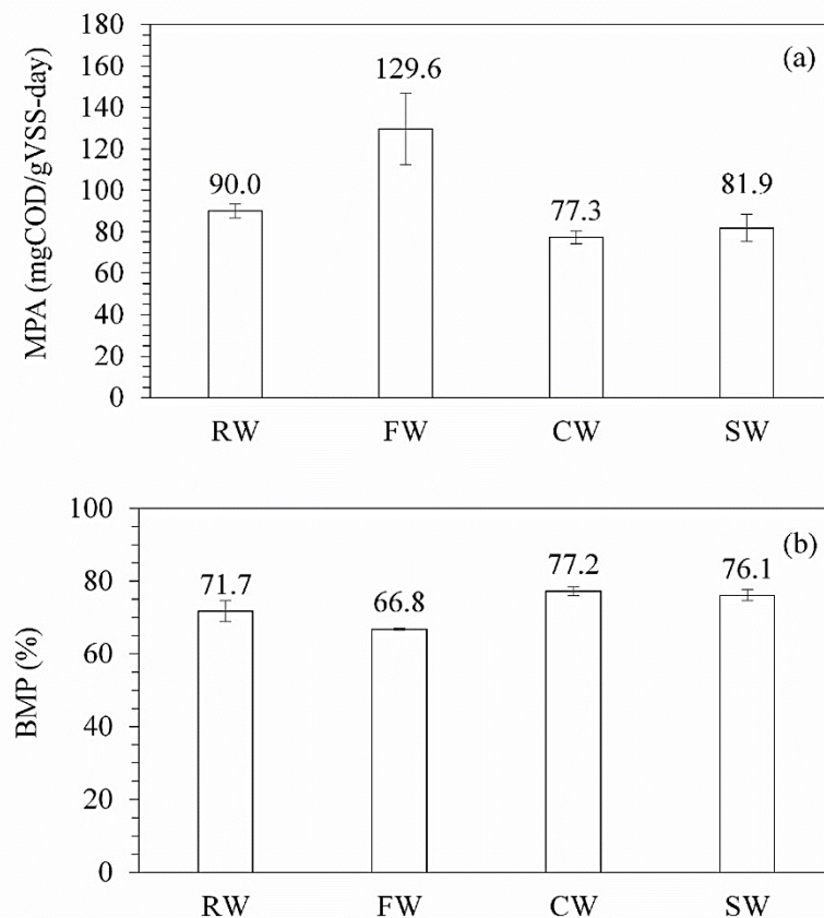
Figure 2 Comparison of (a) MPA and (b) BMP values among the four different wastewater types
