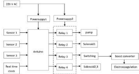
Fig.7 microcontroller input-output diagram
