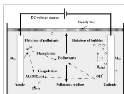
Fig.4 Principle of electrocoagulation
