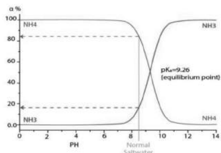
Fig.2 effect of pH to ammonia transform
