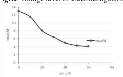
Fig. 16 Current level of electrocoagulation
