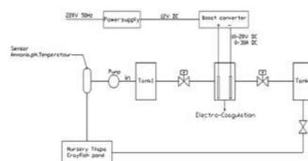
Fig.5 diagram of electrocoagulation system
