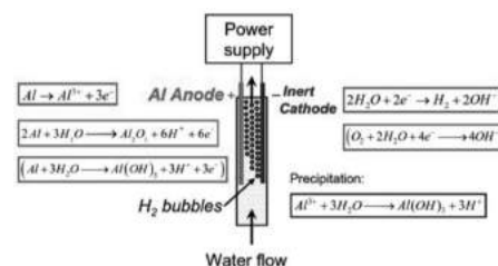
Fig.4 Redox–Oxidation of electrocoagulation
