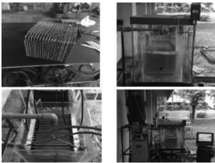
Fig.8 experimental of electrocoagulation
