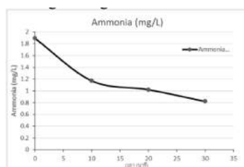
Fig.10 ammonia content from 1.9 mg/L at different reaction times
