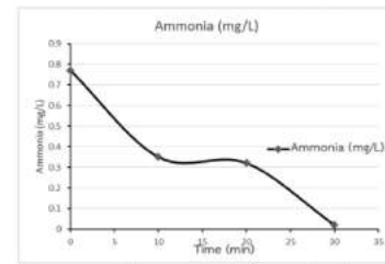
Fig.11 ammonia content from 0.78 mg/L at different reaction times
