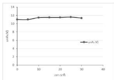
Fig.15 Voltage level of electrocoagulation
