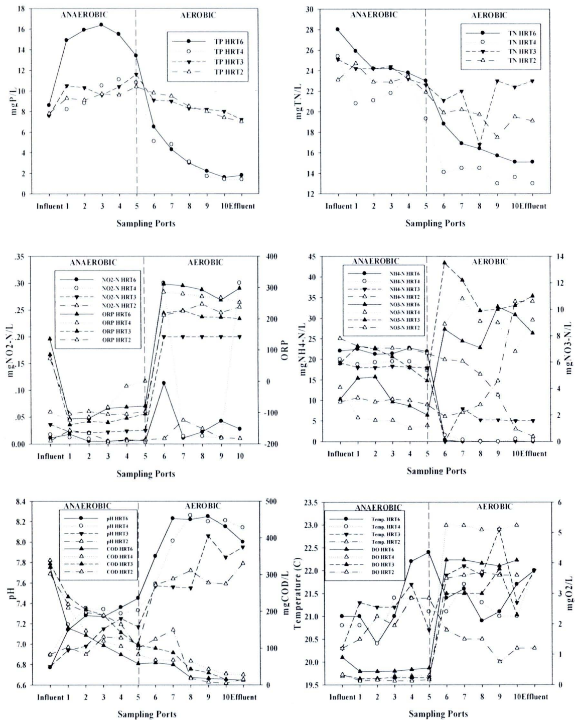
Figure 4.4 Effect of CD of 12 hrs under different HRTs on (a) phosphorus release and uptake, (b) TN removal, (c) changes in ammonia and nitrate concentrations, (d) nitrate and ORP changes, (e) pH changes and COD removal, and (f) changes in temperature and DO with media depth
