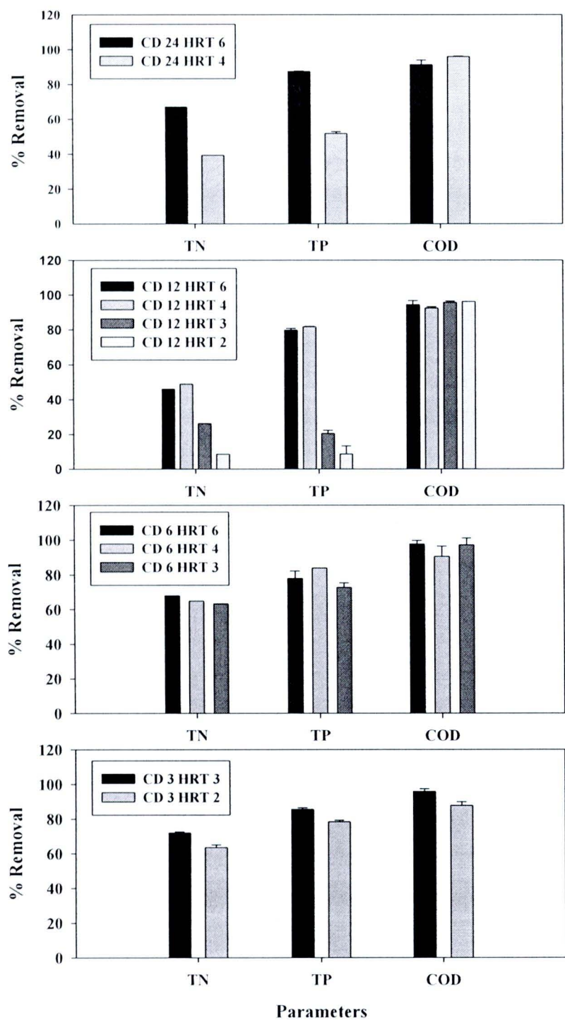
Figure 4.2 Overall percent removals of TP, TN, and COD for a CDs and various HRTs
