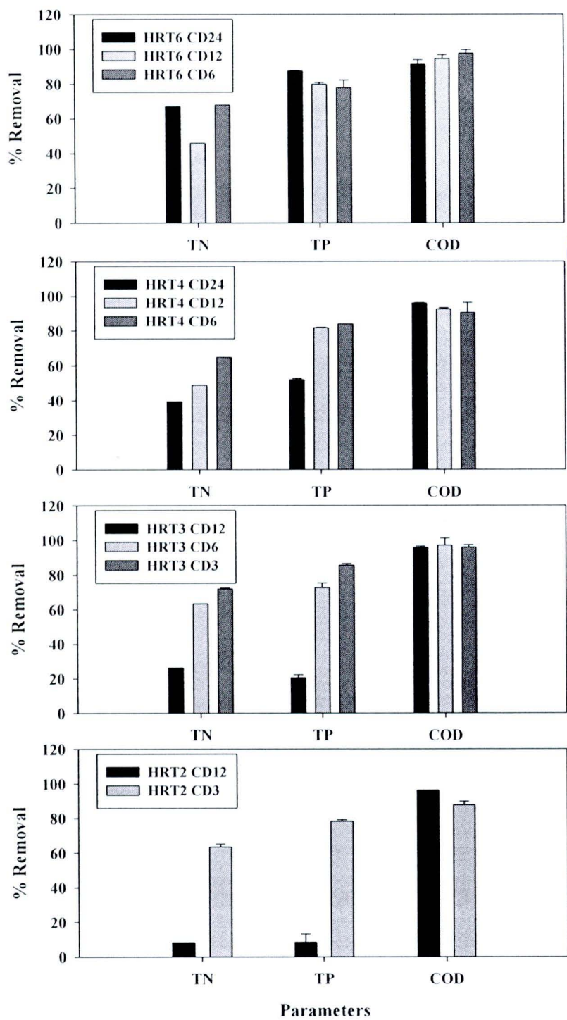
Figure 4.1 Overall percent removal of TP, TN, and COD for a given HRT and various CDs
