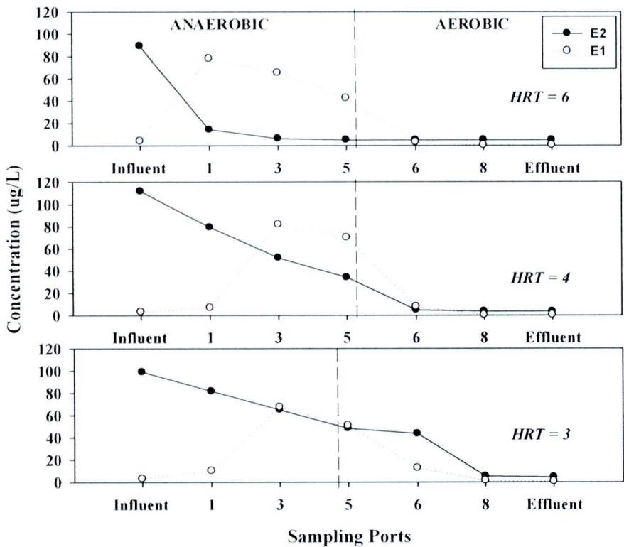
Figure 4.13 E2 removals under different HRTs under anaerobic and aerobic conditions by media depth
