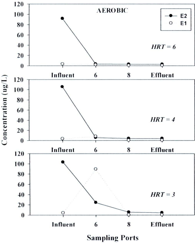
Figure 4.16 E2 removals in aerobic biofilter with media depth.
