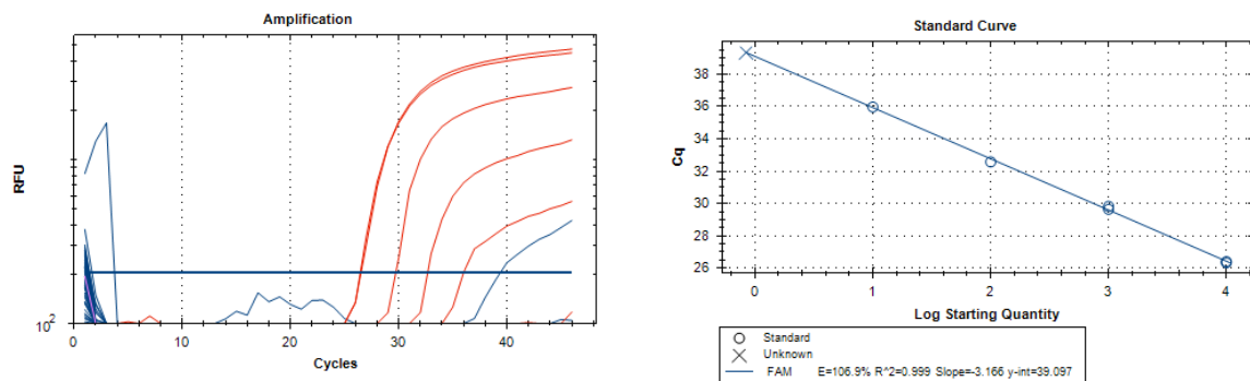
Figure2 Positive qMAL PCR detection in two An. barbirostirs complex. Red lines are STD 10000 copy, 1000 copy, 100 copy, 10 copy. Blue curve lines are positive unknown samples with the over cut off range (bold horizontal blue line). Right graph pictures are standard curve that used for calculate of the copy numbers of PCR products.
