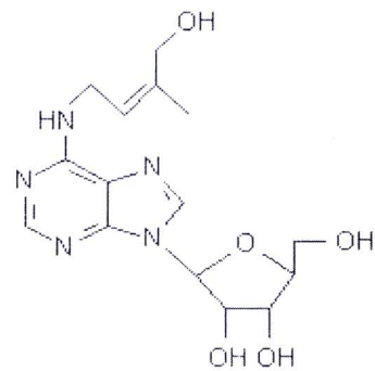
cis -zeatin riboside
