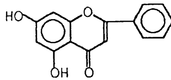
chrysin (2)
