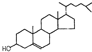
\beta -sitosterol (3)
