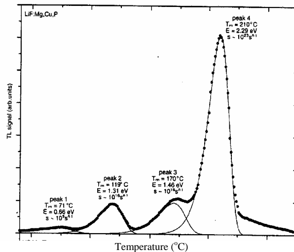
Figure 1.3 Glow curve of LiF: Mg,Cu,P detectors (pre-irradiation annealed at 240 °C for 10 minutes, heating rate 2^\circ\text{C}\cdot\text{s}^{-1} , D = 1.5 mGy) (25).
