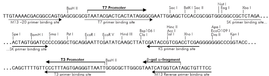
Figure 6 Physical map of pBluescript-HAC1b
