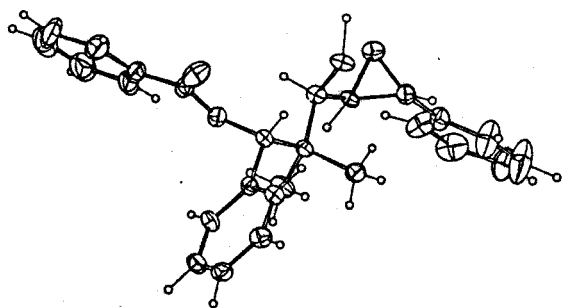
Fig. 1 ORTEP drawing of compound 5a
