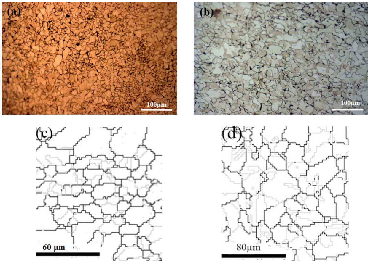
Fig.2. Microstructure and Grain boundary reconstruction images of base metal - BM (a,c) and as-recrystallized – As-ReX (b,d). Grey lines indicate \Sigma 3-29 boundaries and black lines represent \Sigma > 29
