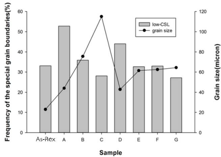
Fig. 4. The fraction of special grain boundary with grain size in each sample
