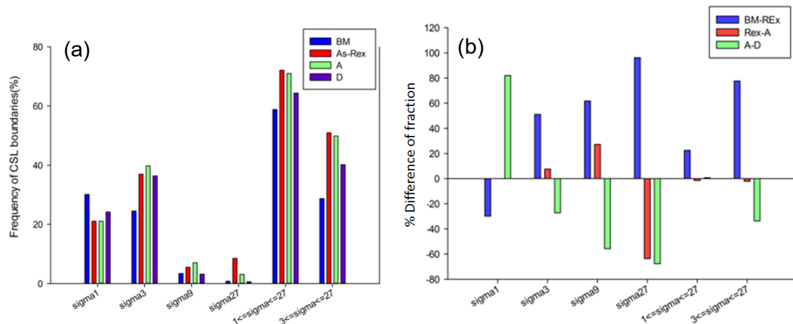
Fig. 3. The Fraction of special boundary of iterative recrystallized sample (a) and % different of fraction of processed samples with respected to former recrystallized samples.
