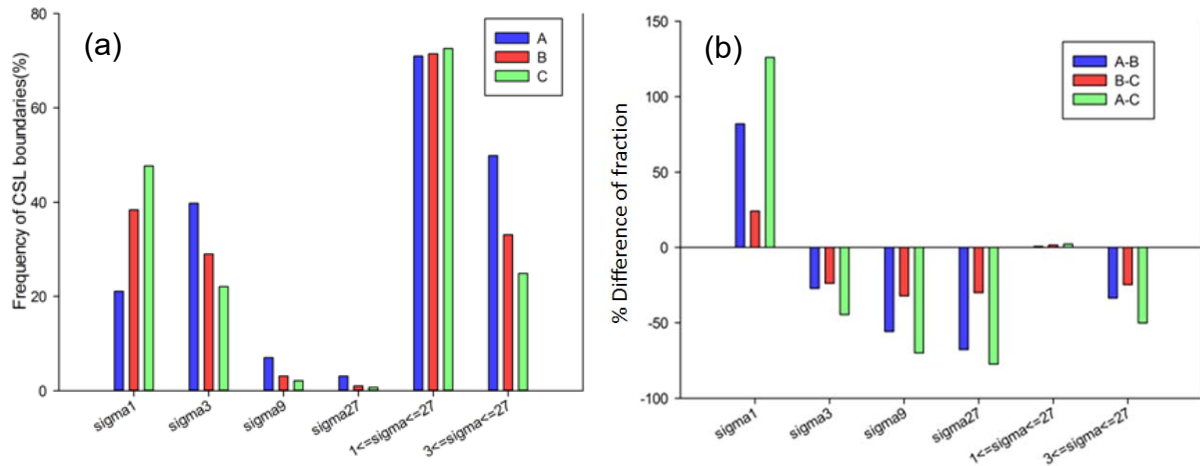
Fig. 5. The Fraction of special boundary of sample A, B, C (a) and % difference of fraction of processed samples with respected to the smaller grain size sample.
