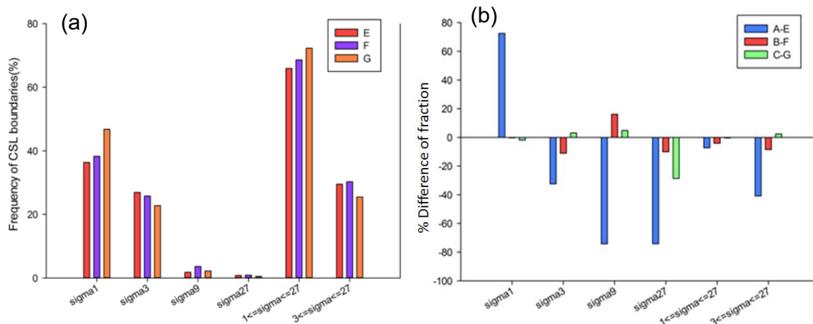
Fig. 5. The Fraction of special boundary of 3 rd recrystallized samples (a) and % difference of fraction of each processed sample with respected to its own initial 2 nd recrystallized samples.
