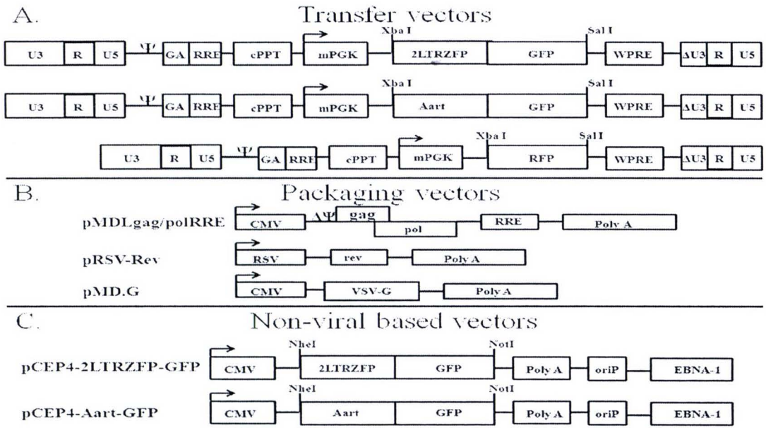
Figure 3.12 Schematic drawing of the expression vectors for 2LTRZFP-GFP, Aart-GFP, and RFP. (A) The transfer vectors used in this study were derived from the third-generation, self-inactivating vector pRRLSIN.cPPT.mPGK-GFP.WPRE. The Xba I and Sal I sites were used as the cloning sites for all transgenes. The following abbreviations are used: cPPT, central polypurine tract; GA, fragment of the HIV-1 gag gene; RRE, Rev responsive element; and WPRE, woodchuck hepatitis virus post-transcriptional regulatory element. (B) The packaging vector, pMDLgag/polRRE, expresses the gag and pol transcript, intervening sequences and polyadenylation site, and it is driven by the CMV promoter. pRSV-Rev expresses rev cDNA. pMD.G encodes a heterologous envelope to pseudotype the virus coding for VSV-G. (C) The non-viral based vector, pCEP4, was used to construct pCEP4-2LTRZFP-GFP and pCEP4-Aart-GFP for stable cell line production. Nhe I and Not I were used as cloning sites for both transgenes. The EBV origin of replication (oriP) and nuclear antigen (EBNA-1) signal result in high-copy episomal replication in primate and canine cell lines (Yates et al., 1985; Reisman and Sugden, 1986).
