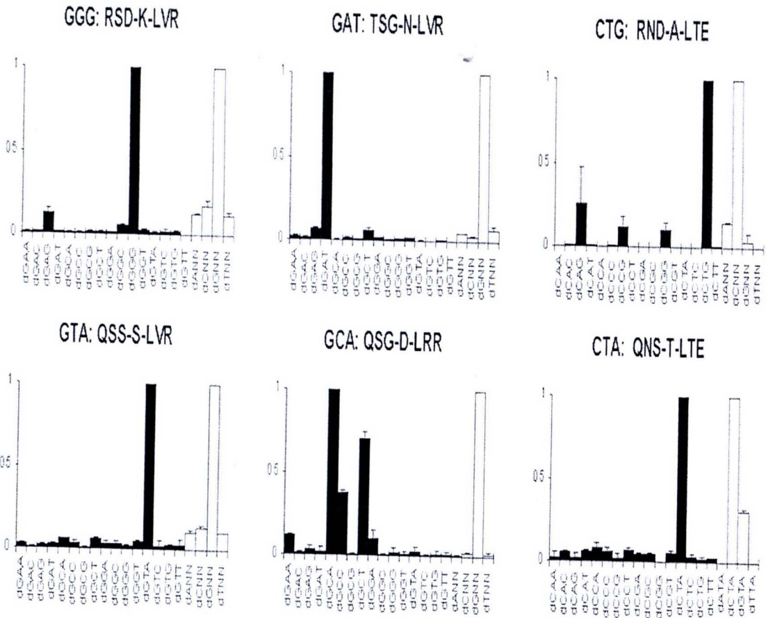
Figure 3.1 The pop-up ELISA graphs for predicted binding activity in each finger to triplet DNA target (Segal et al., 1999; Dreier et al., 2000; Mandell and Barbas, 2006). At the top of each graph is the recognition helix for each finger (positions -1 to 6). Position 3 is flanked by dash marks (-) for clarity. Black bars represent the binding activity of each finger with target oligonucleotides. White bars represent the binding activity of each finger with oligonucleotide pools with a particular 5' nucleotide subsite: GNN, ANN, TNN, and CNN. The height of each bar represents the relative specificity of the protein for each target, averaged over two independent experiments and normalized to the highest signal among the black or white bars. Error bars represent the deviation from the average.
