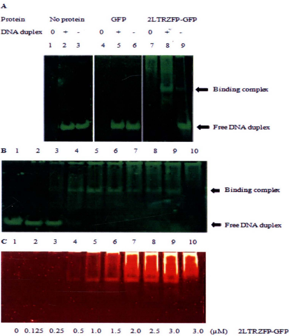
Figure 3.11 Electrophoretic mobility shift assay (EMSA). (A) The protein used for each reaction is 1 μM whereas [0], no DNA duplex; [+], specific DNA duplex; [-], non-specific DNA duplex. The gel was stained with SYBR® Green EMSA stain (B) or with SYPRO® Ruby EMSA stain (C). In panel B and C: Lane 1 to 9, the specific DNA duplex used for each reaction was 250 nM, whereas 2LTRZFP-GFP was varied the concentration from 0, 0.125, 0.25, 0.5, 1.0, 1.5, 2.0, 2.5, 3.0 μM, respectively. Lane 10, 2LTRZFP-GFP was used 3.0 μM, but no DNA duplex.
