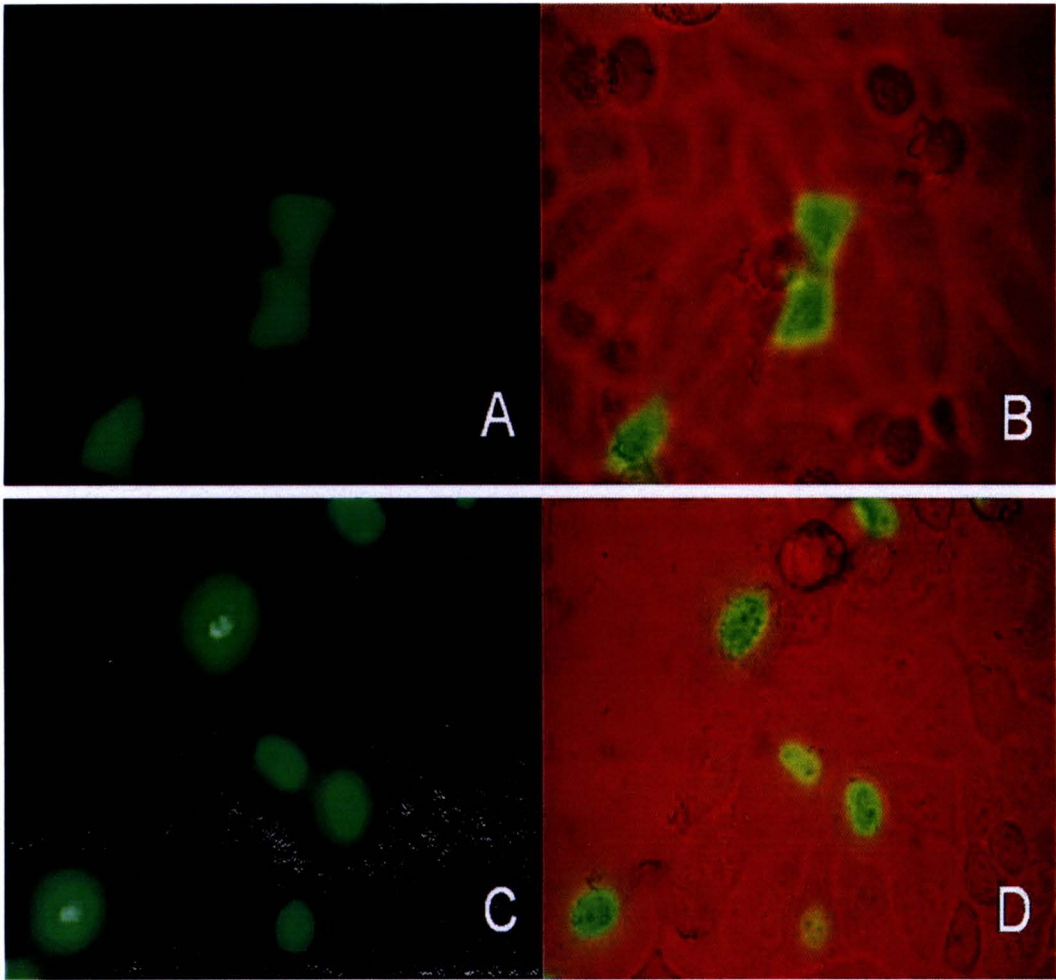
Figure 3.7 Expression of green fluorescent protein in HeLa cells 24 h after transfection. (A and B) Transfected with recombinant plasmid pTriEx-4-GFP. (C and D) Transfected with recombinant plasmid pTriEx-4-2LTRZFP-GFP. Each group was imaged at 400 \times magnification in the same field by inverted fluorescent microscope.
