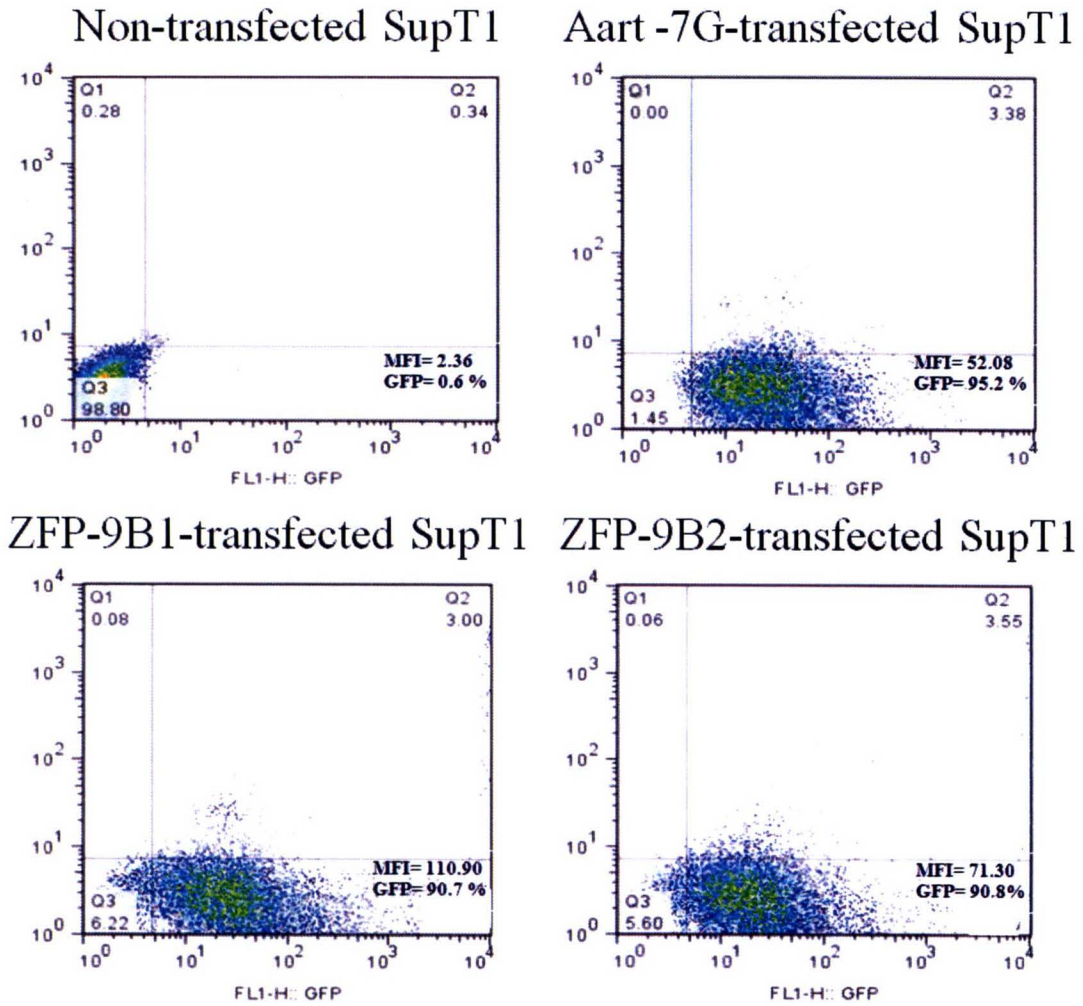
Figure 3.24 GFP expression in SupT1 cells stably transfected with either 2LTRZFP-GFP or Aart-GFP. Cells that expressed 2LTRZFP-GFP or Aart-GFP were monitored GFP by flow cytometry. MFI; mean fluorescence intensity.
