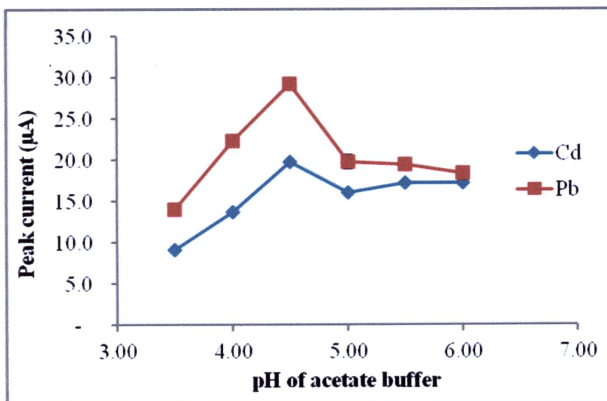
Figure 3.2 Effect of pH on metal decumulation at electrode ( 20 \mu\text{g/L} each of Cd(II) and Pb(II)). Experimental conditions: 0.10 M acetate buffer containing 0.50 mg/L Bi(III), deposition potential -1.5 V, deposition time of 90 s, cleaning potential of 0.6 V, cleaning time of 60 s, equilibration time of 30 s, voltage step of 6 mV, amplitude of 50 mV frequency 50 Hz and flow rate of the sample or standard solution at 0.5 ml/min.
