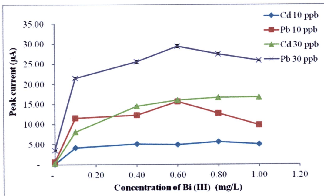
Figure 3.3 Effect of \text{Bi(III)} concentration (10 and 30 \mu\text{g/L} each of \text{Cd(II)} and \text{Pb(II)} ). Experimental conditions: 0.10 M acetate buffer pH 4.5, deposition potential -1.5 V, deposition time of 90 s, cleaning potential of 0.6 V, cleaning time of 60 s, equilibration time of 30 s, voltage step of 6 mV, amplitude of 50 mV frequency 50 Hz and flow rate of the sample or standard solution at 0.5 ml/min.
