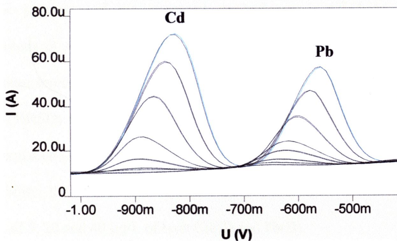
Figure 3.8 Square wave anodic stripping voltammograms obtained from VA-BiFE system of solution containing Cd(II) and Pb(II) of increasing concentration, from 2-40 \mu\text{g/L}
