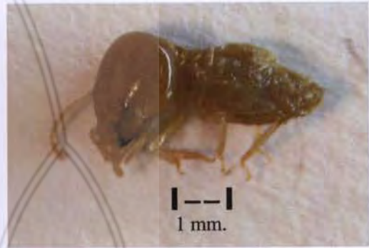
Coptotermes curvignathus
