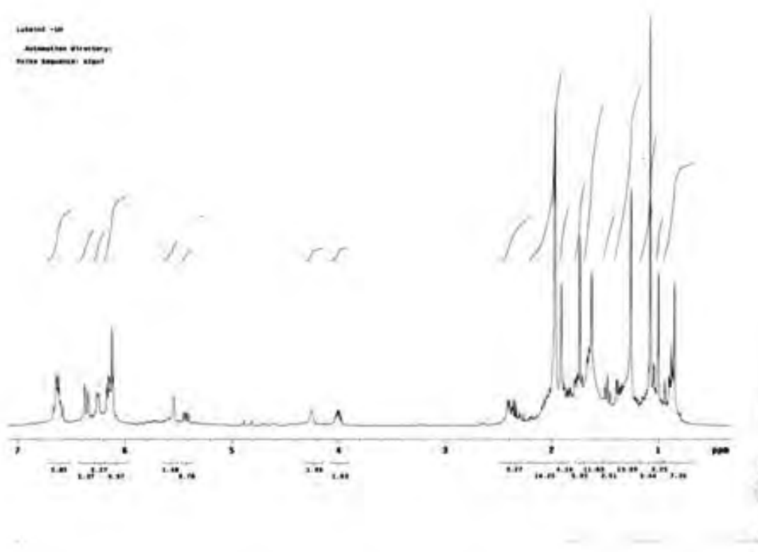
Fig. 5. H-NMR chromatograms of lutein sample after chromatographic purification.
