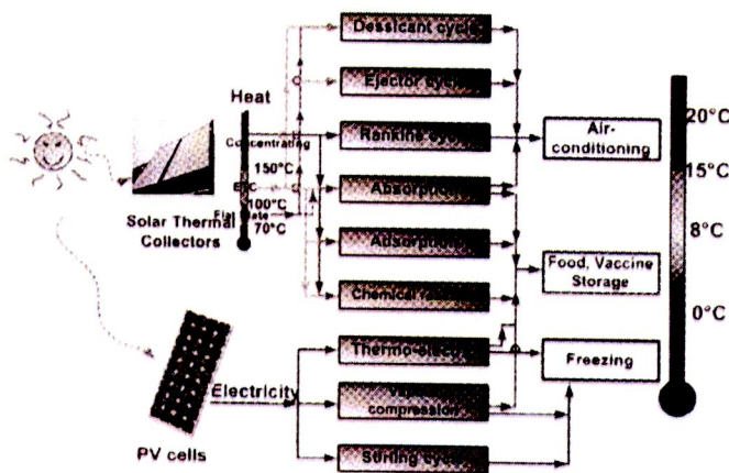
Figure 2.3 Solar cooling paths (Pridasawas, 2006).
