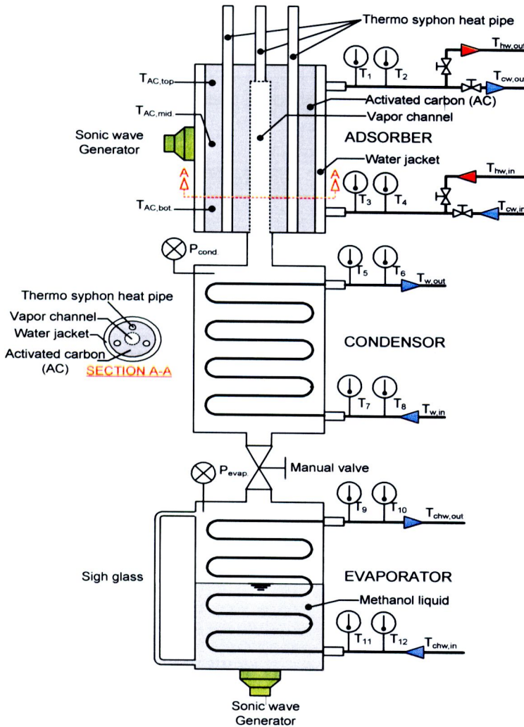
Figure 2.4 schematic sketches of the experiment apparatus.
