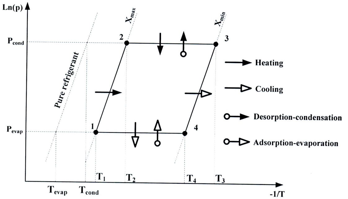
Figure 2.2 P - T - x diagram of an adsorption cycle.
