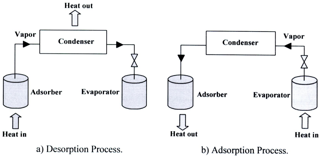
Figure 2.1 Basic operating principle of adsorption process.
