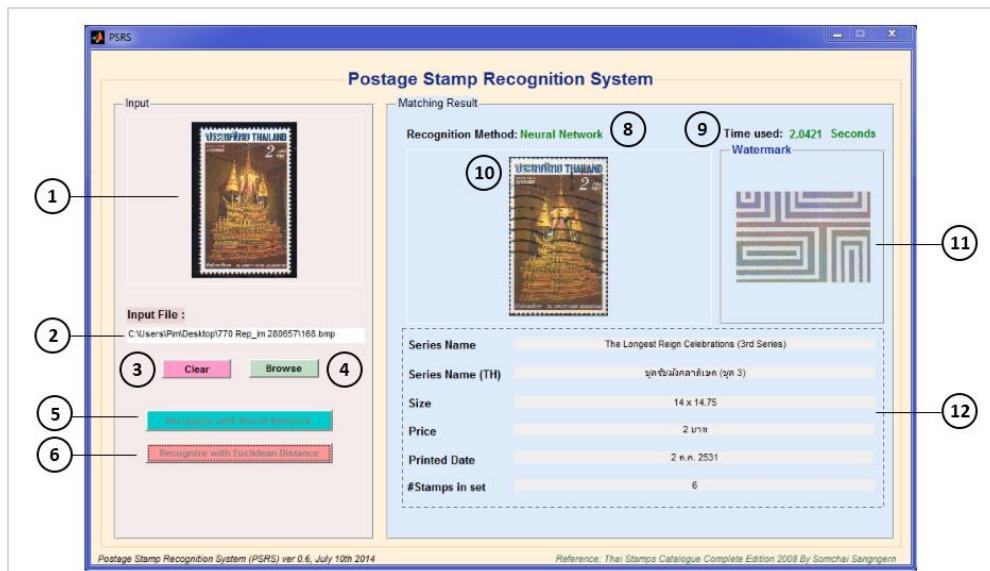
Figure 3-16 PSRS Interface Design (2)
