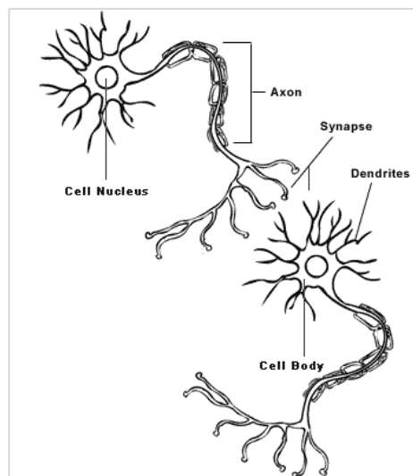
Figure 3.21 Biological Neuron
