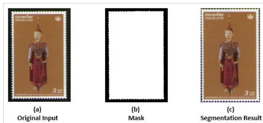
Figure 3.11 Segmentation Result
