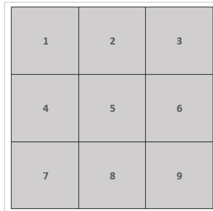
Figure 3.12 Region Layout
