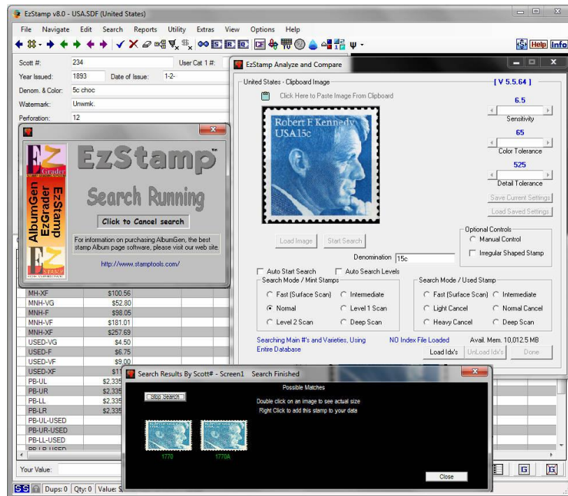
Figure 2.6 SRS Interface [7]
