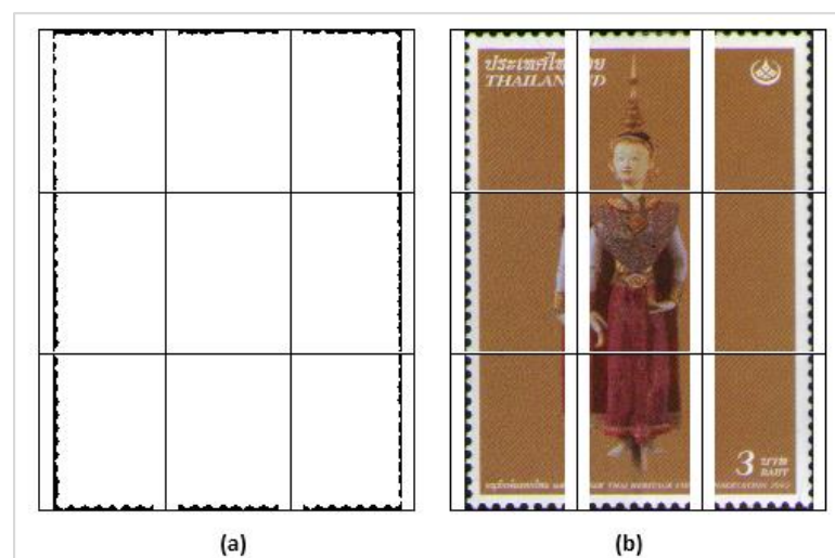
Figure 3.13 Division Result
