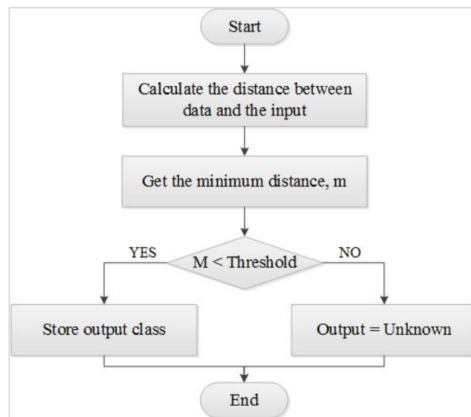
Figure 4.16 Euclidean Distance Flowchart
