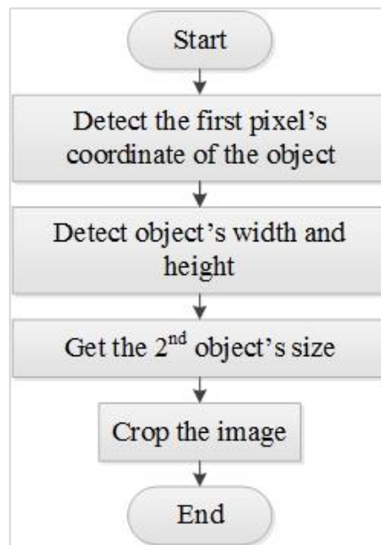
Figure 4.10 Object Segmentation Flowchart
