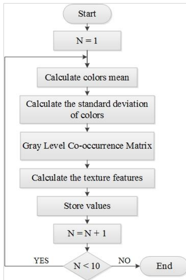
Figure 4.14 Features Extraction Flowchart
