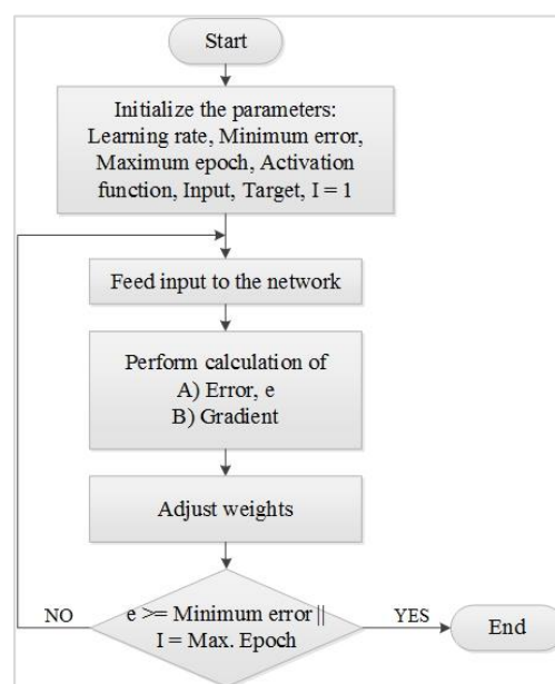
Figure 4.18 Training ANN Flowchart
