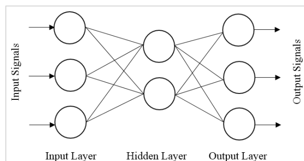
Figure 3.22 ANN Architecture
