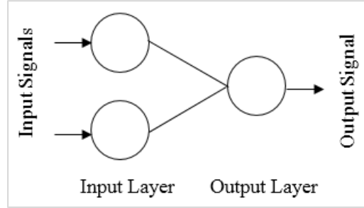
Figure 3.23 Two-input Perceptron
