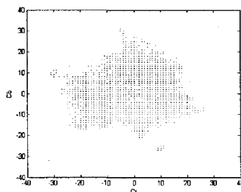
Figure 2.3 C_b and C_r Graph [4]
