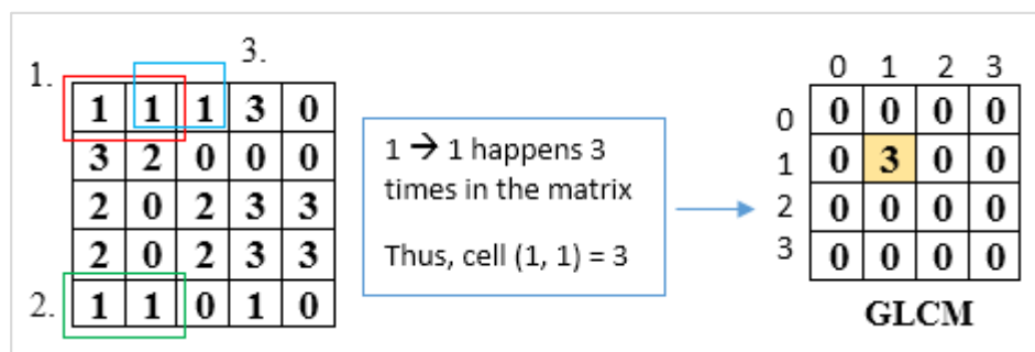
Figure 3.18 GLCM Calculation
