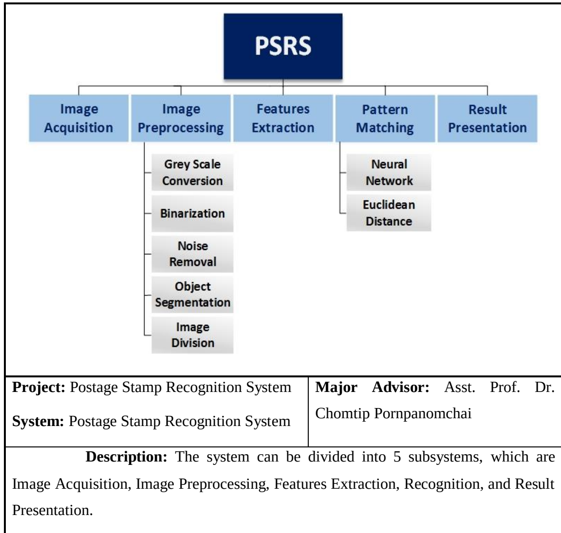
Figure 3.2 PSRS Structure Chart
