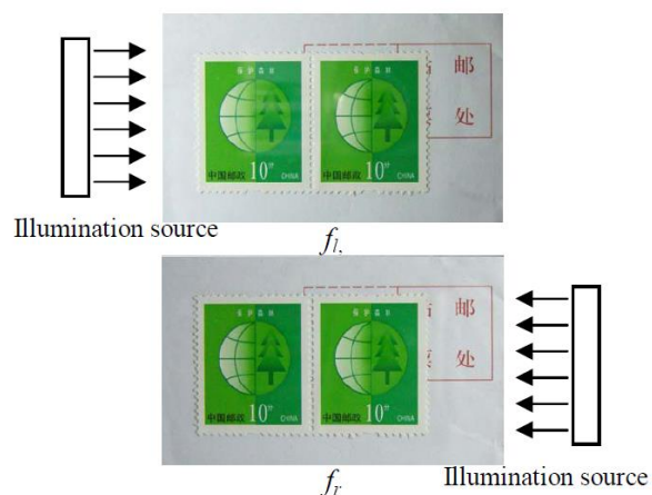
Figure 2.1 The RGB image produced by two Illumination sources [3]
