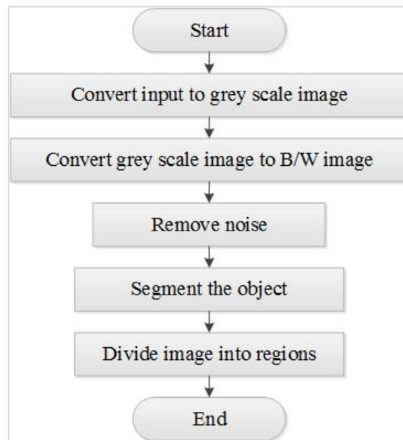
Figure 4.3 Preprocessing Flowchart
