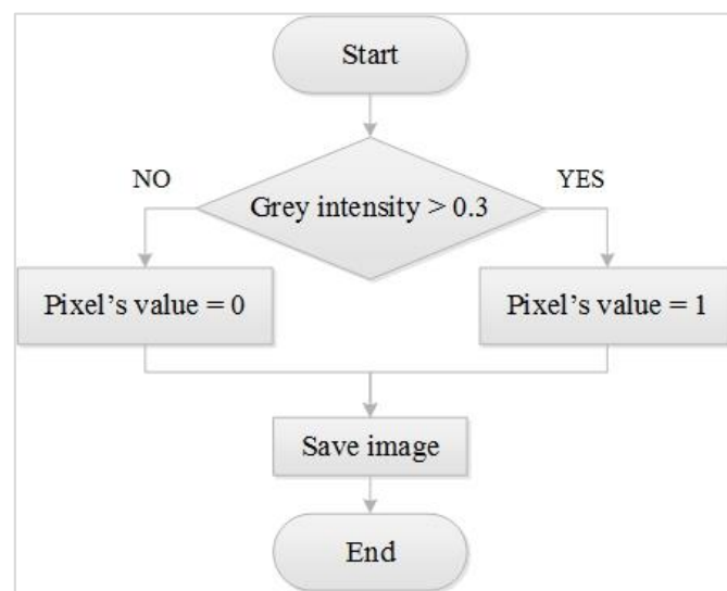
Figure 4.6 Binarization Flowchart
