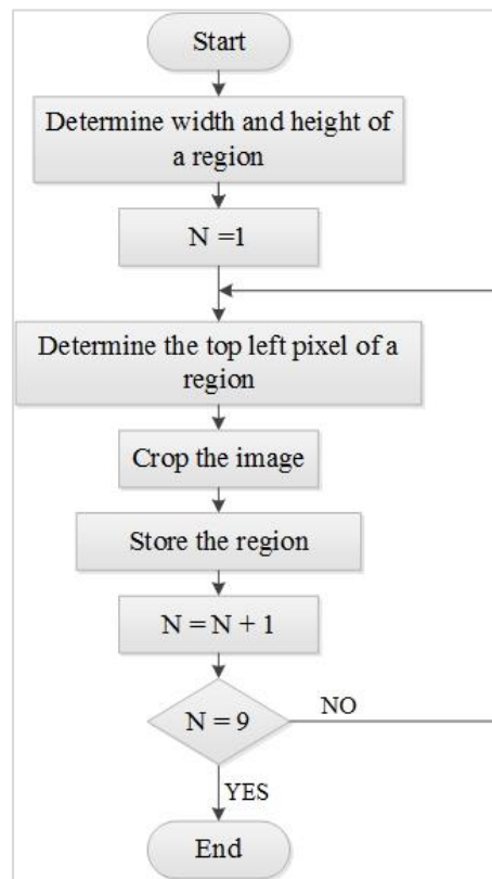
Figure 4.12 Image Division Flowchart
