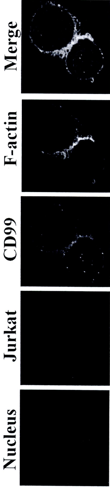
Figure 3.26 CD99 is recruited into the IS
