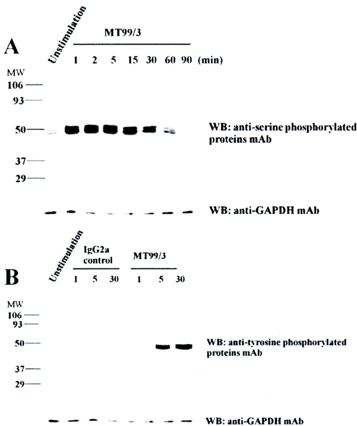
Figure 3.31 Analysis of protein serine phosphorylation upon CD99 engagement. Serum starved Jurkat cells were treated with anti-CD99 mAb MT99/3 for 30 mins and then cross-linking with goat anti-mouse IgG for the indicated time periods. Phosphorylation levels of the various signaling molecules in cell lysates were determined by immunoblotting analyses using specific antibodies for serine phosphorylated proteins. (A) Serum starved Jurkat cells were treated with anti-CD99 mAb MT99/3 for 30 mins and then cross-linking with goat anti-mouse IgG for the indicated time periods. (B) Serum starved Jurkat cell lysate treated with mAb MT99/3 and isotype matched control mAb for 30 mins and then with goat anti-mouse IgG for the indicated time periods. Immunoblotting against GAPDH serve as a control for equal protein loading.
