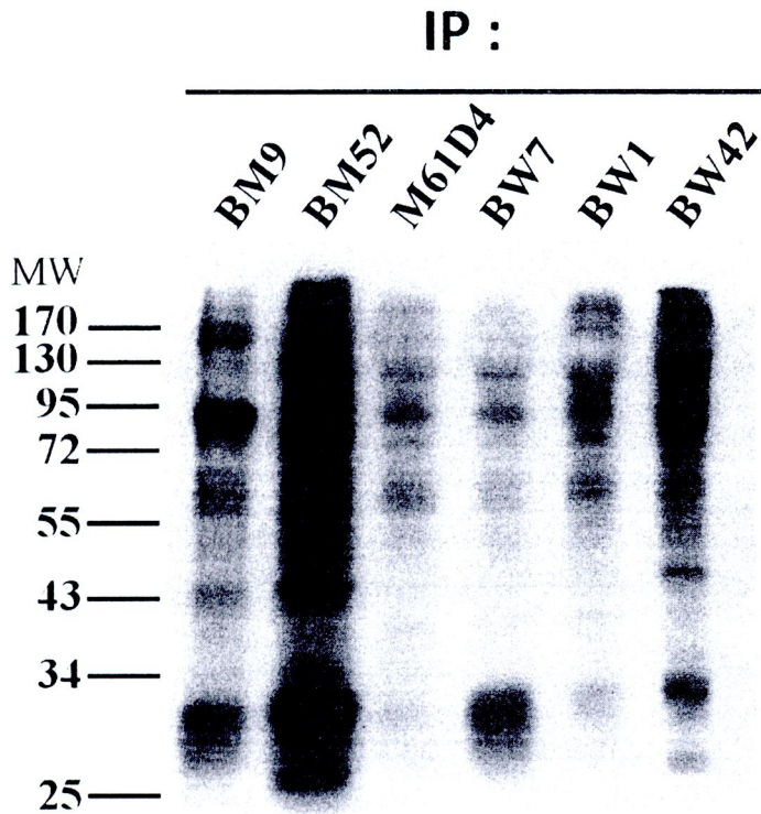
Figure 3.18 Verification of the interaction between the proteins recognized by the generated mAb and CD99 molecules
