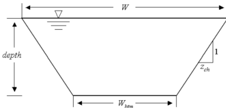
Figure 7:1-1: Trapezoidal channel dimensions
