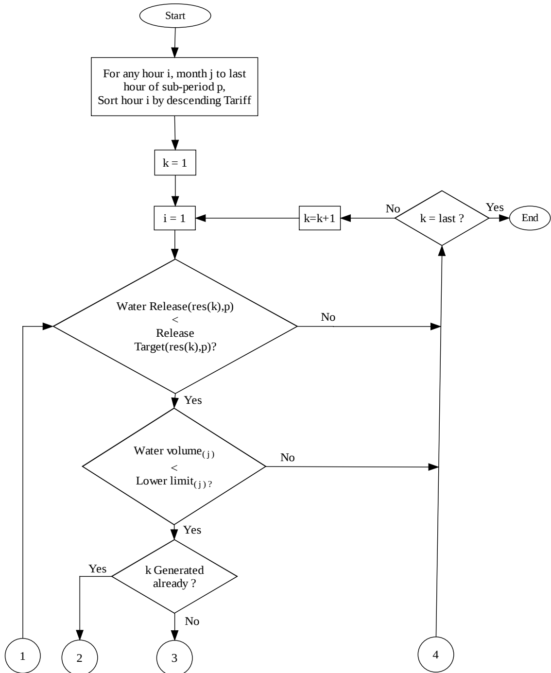
Figure 3.4 Generation to meet Water Release in sub-period flow chart.
