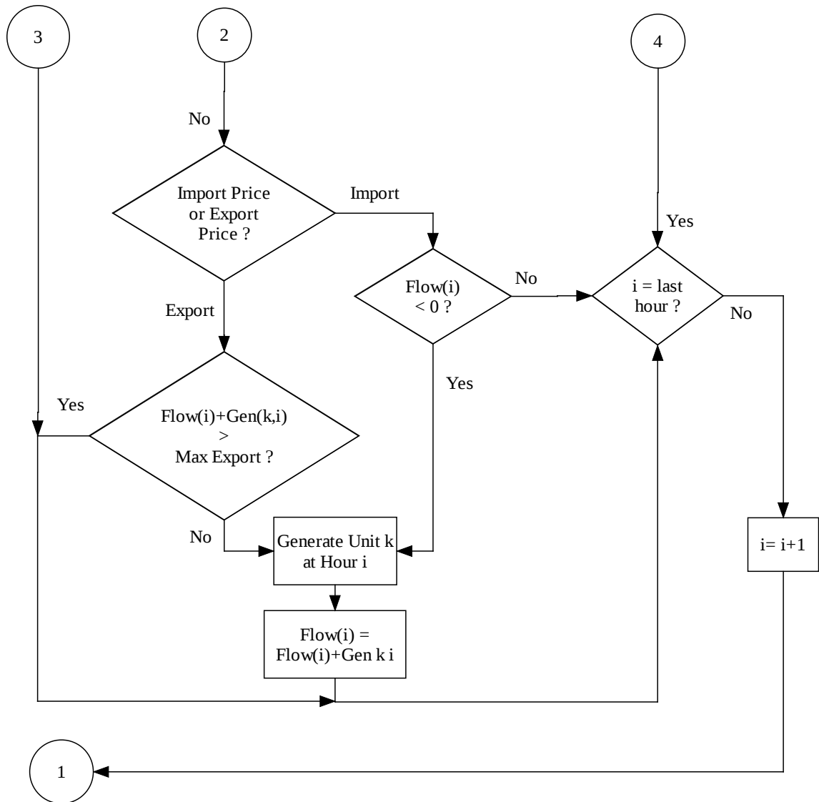
Figure 3.3 Flow chart of Generation to meet Minimum Release of each month (Continue)
