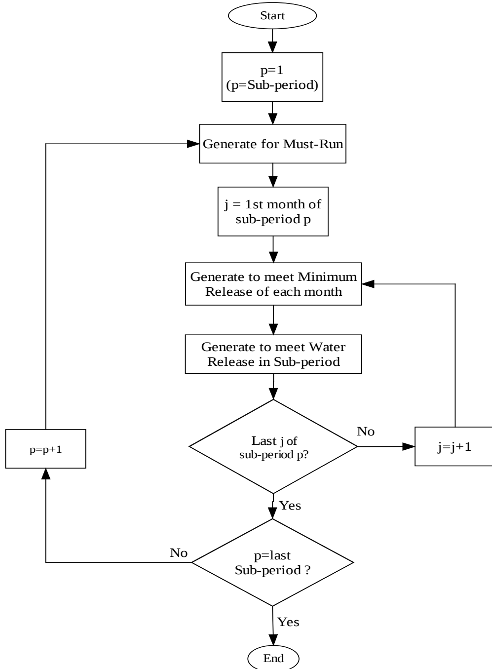
Figure 3.2 Generation planning flow chart for each reservoir
