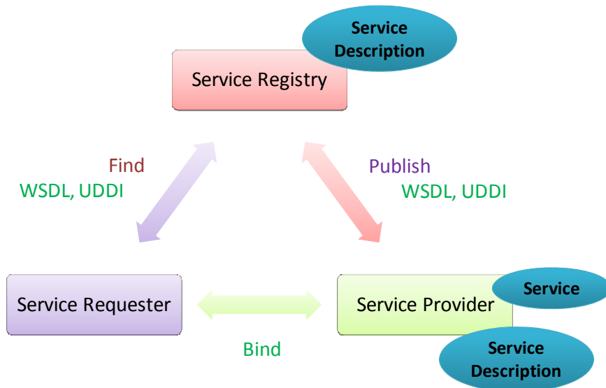
Figure 3.1 Web Services Model
