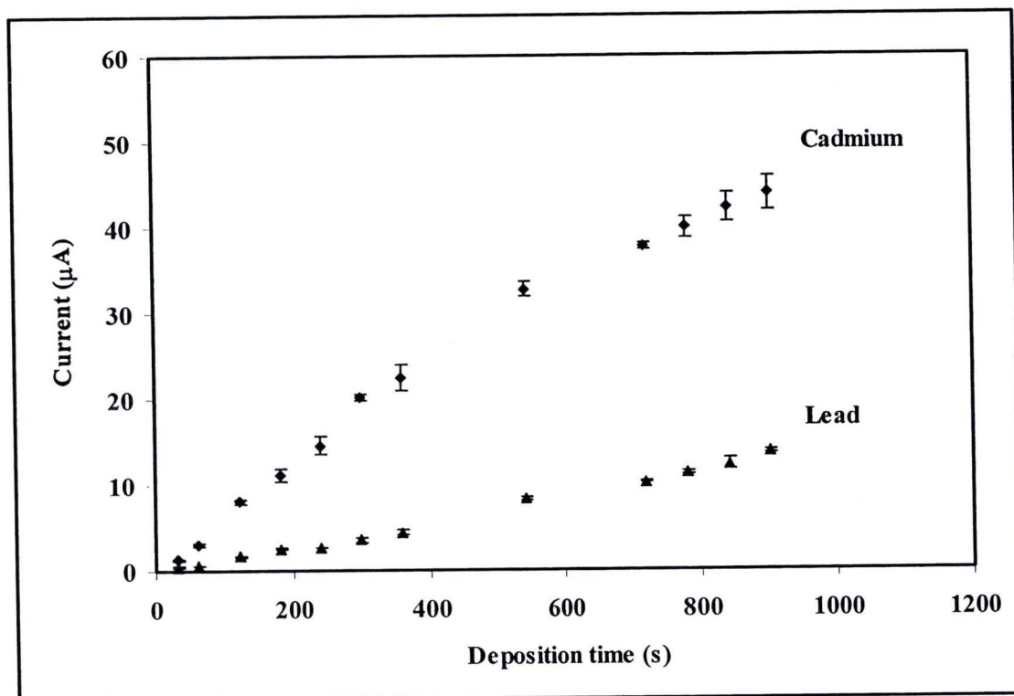
Figure 4.12 Effect of the deposition time on the stripping peak currents for 25 \mu\text{g}\cdot\text{L}^{-1} of cadmium (II) and lead (II) ions in 0.1 M acetate buffer solutions (pH 4.5) recorded with in situ BiF/CNT/GC electrodes by SWASV using the same experimental conditions as those in Fig. 4.9.
