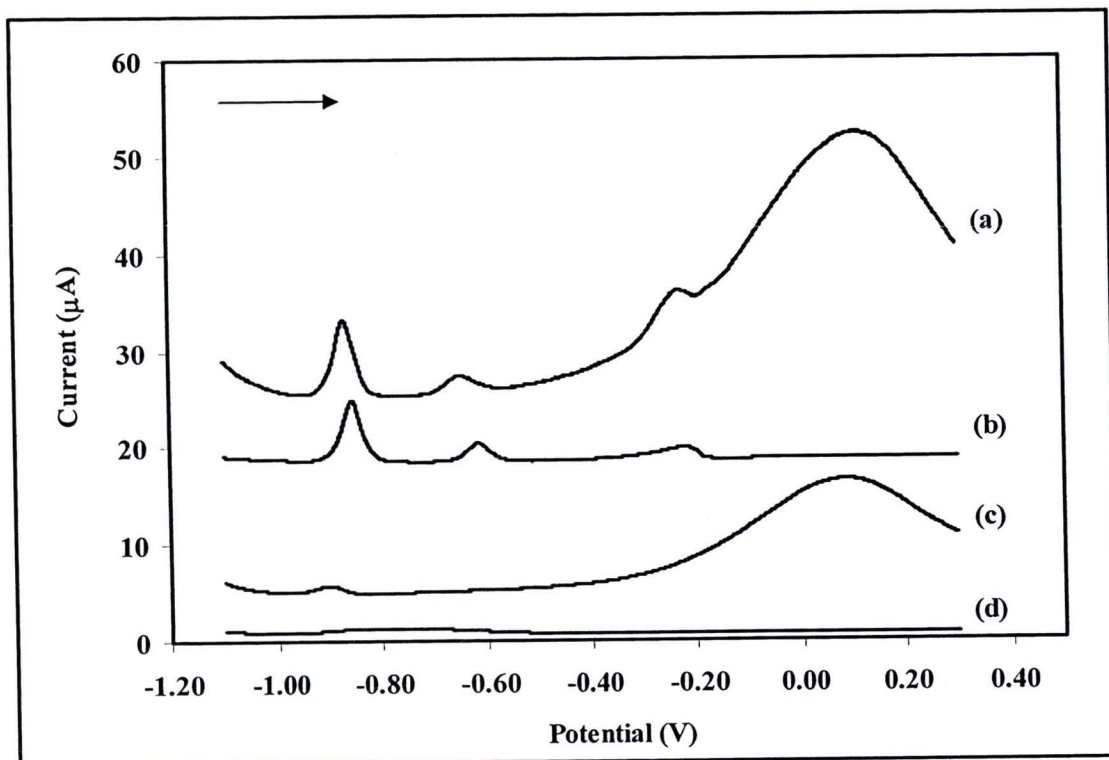
Figure 4.7 SWASV voltammograms for 0.1 M acetate buffer solution (pH 4.5) containing 25 \mu\text{g}\cdot\text{L}^{-1} of cadmium (II) and lead (II) ions recorded with (a) in situ BiF/CNT/GC electrode, (b) in situ BiF/GC electrode, (c) CNT/GC electrode, and (d) GC electrode with the deposition potential of -1.10 \text{ V} , the deposition time of 120 s, and the scan rate of 7.5 \text{ mV}\cdot\text{s}^{-1} .
