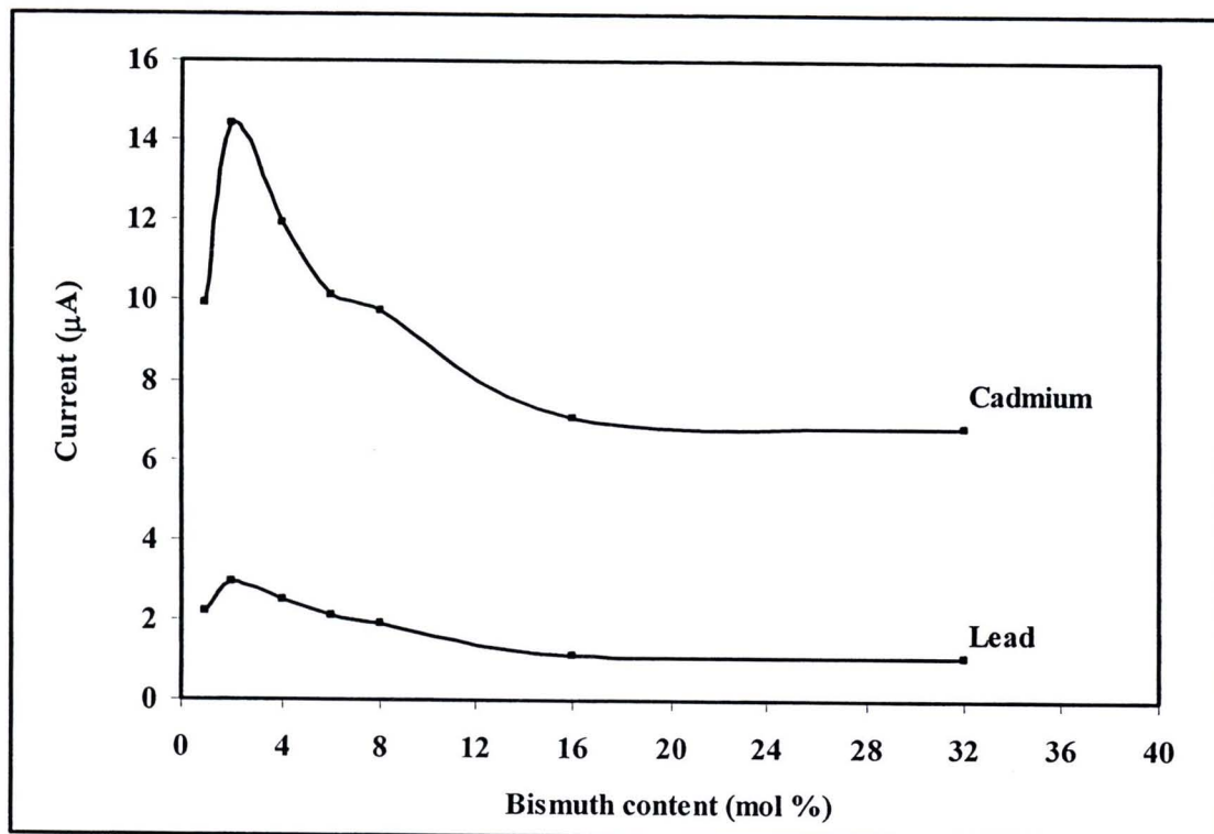
Figure 4.17 Effect of bismuth content in Bi–CNT composite on the stripping voltammetric responses for 25 \mu\text{g}\cdot\text{L}^{-1} of cadmium (II) and lead (II) ions in 0.1 M acetate buffer solutions (pH 4.5) recorded with Bi–CNT/GC electrodes by SWASV using the same experimental conditions as those in Fig. 4.15.
