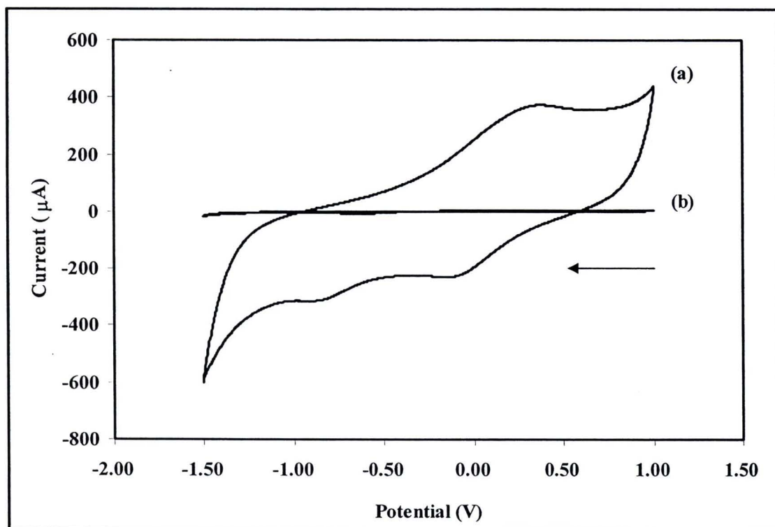
Figure 4.6 Cyclic voltammograms for 0.1 M acetate buffer solution (pH 4.5) recorded with (a) CNT/GC electrode and (b) bare GC electrode at the scan rate of 100 \text{ mV} \cdot \text{s}^{-1} .
