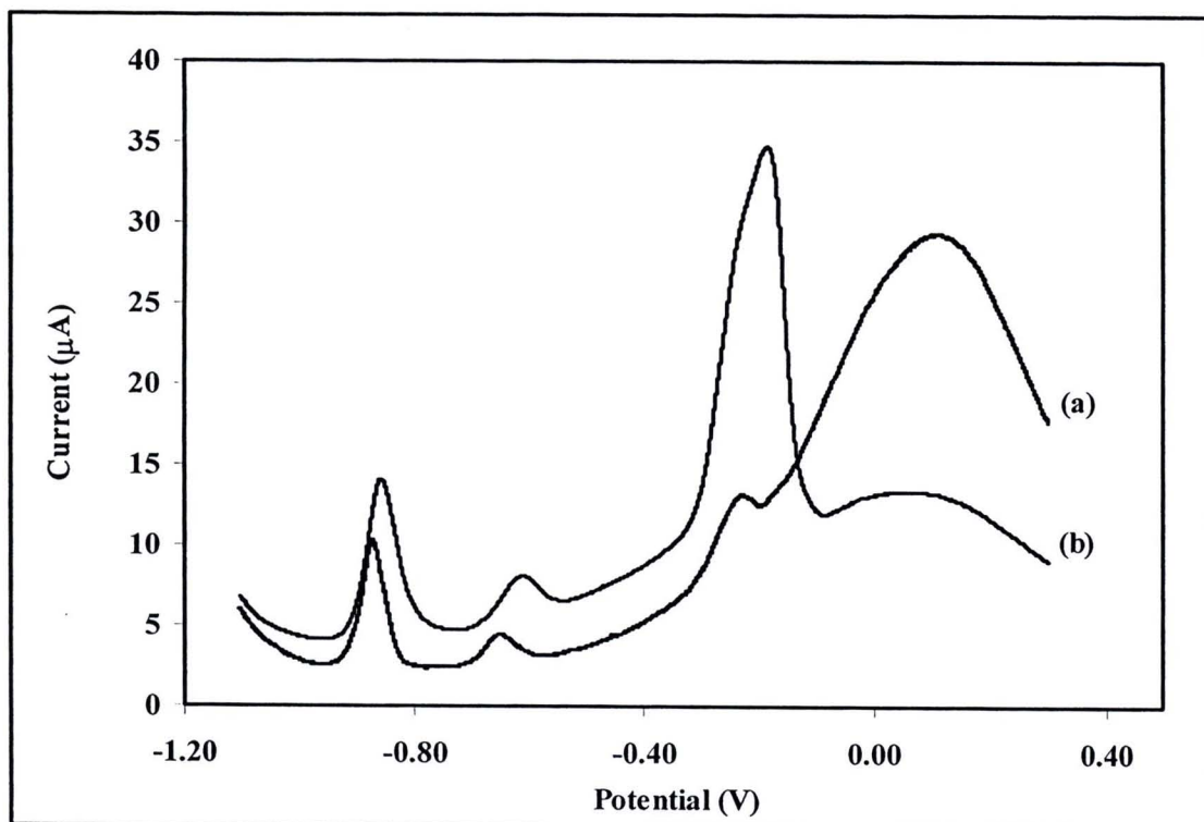
Figure 4.15 SWASV signals obtained from (a) in situ BiF/CNT/GC electrode and (b) 2.00 mol % Bi–CNT/GC electrode for 0.1 M acetate buffer solution (pH 4.5) containing 25 \mu\text{g}\cdot\text{L}^{-1} of cadmium (II) and lead (II) ions with the deposition potential of -1.10 \text{ V} , the deposition time of 120 s, and the scan rate of 7.5 \text{ mV}\cdot\text{s}^{-1} .
