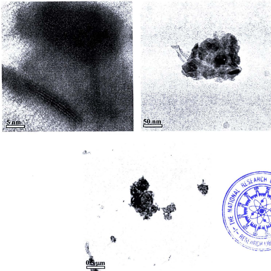
Figure 4.5 TEM images of 4.00 mol % Bi–CNT composite.
