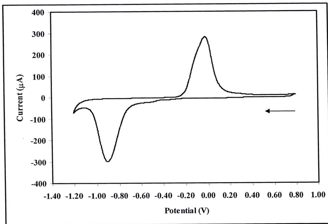
Figure 4.14 Cyclic voltammogram for 0.1 M acetate buffer solution (pH 4.5) recorded with 4.00 mol % Bi–CNT/GC electrode at the scan rate of 100 \text{ mV}\cdot\text{s}^{-1} .
