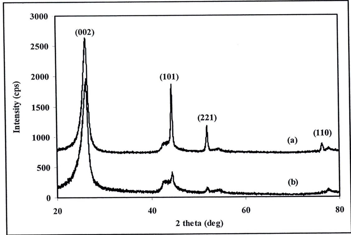
Figure 4.2 XRD patterns of the (a) unmodified and (b) modified CNTs.
