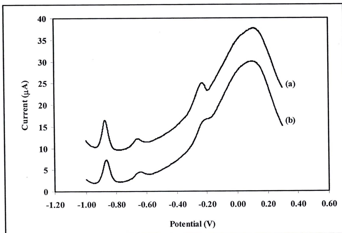
Figure 4.8 SWASV voltammograms for 0.1 M acetate buffer solution (pH 4.5) containing 25 \mu\text{g}\cdot\text{L}^{-1} of cadmium (II) and lead (II) ions recorded with in situ BiF/CNT/GC electrodes in the (a) presence and (b) absence of O_2 using the deposition potential of -1.10 \text{ V} , the deposition time of 120 s, and the scan rate of 7.5 \text{ mV}\cdot\text{s}^{-1} .
