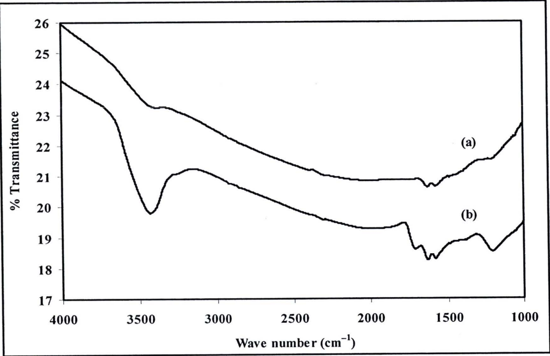
Figure 4.1 FTIR spectra of the (a) unmodified and (b) modified CNTs.
