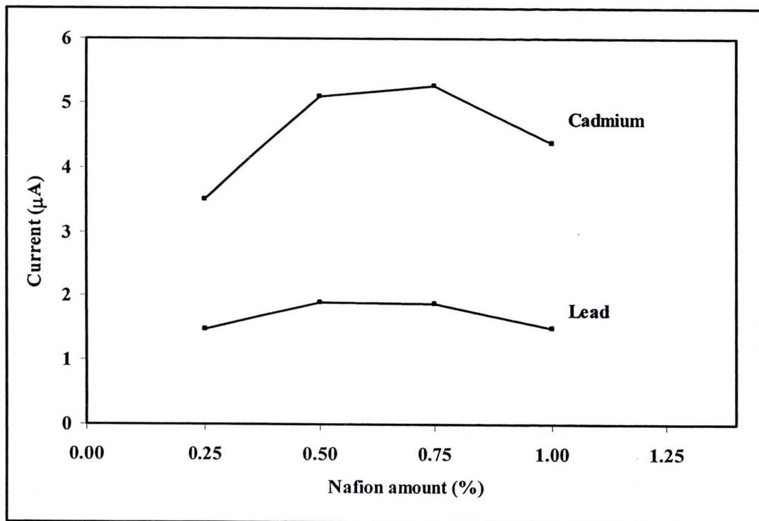
Figure 4.16 Effect of Nafion amount on the stripping currents for 25 \mu\text{g}\cdot\text{L}^{-1} of cadmium (II) and lead (II) ions in 0.1 M acetate buffer solutions (pH 4.5) recorded with Bi-CNT/GC electrodes by SWASV using the same experimental conditions as those in Fig. 4.15.
