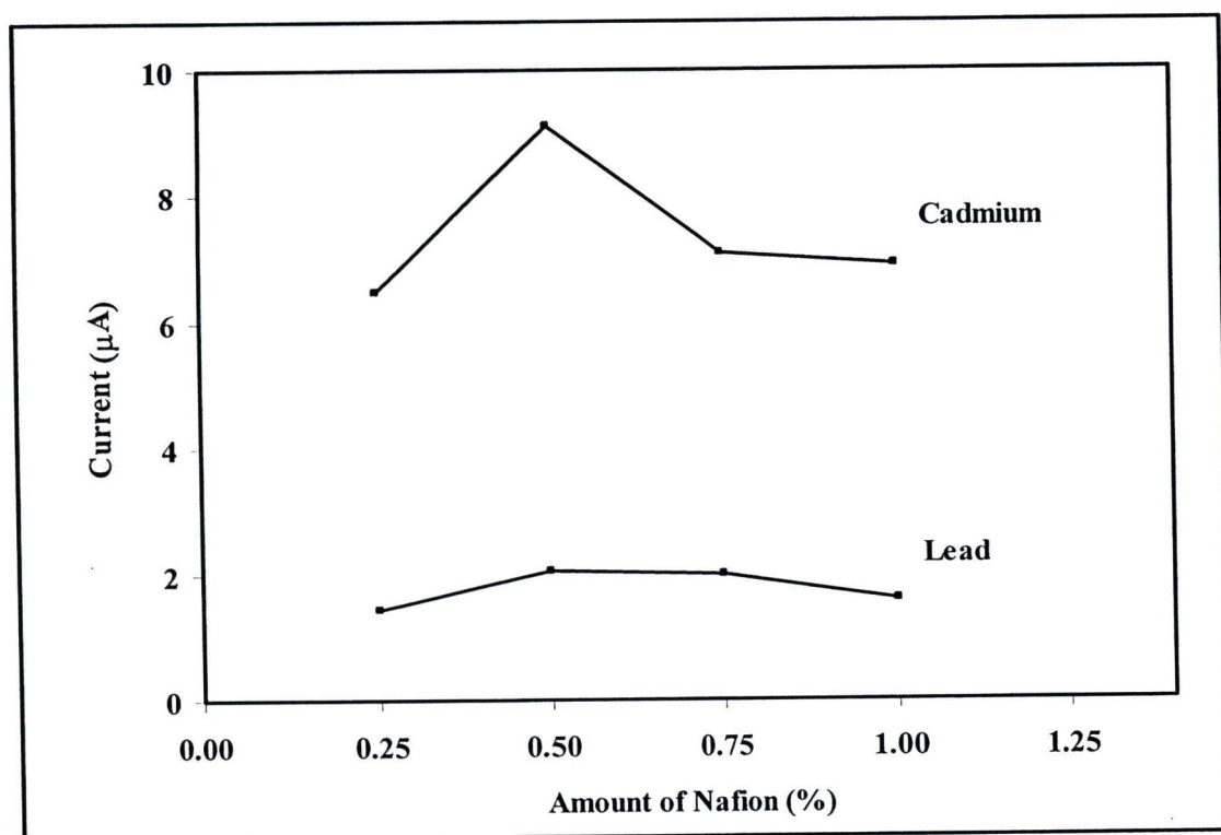
Figure 4.9 Effect of Nafion amount on the stripping peak currents for 25 \mu\text{g}\cdot\text{L}^{-1} of cadmium (II) and lead (II) ions in 0.1 M acetate buffer solutions (pH 4.5) recorded with in situ BiF/CNT/GC electrodes by SWASV using the deposition potential of -1.10 \text{ V} , the deposition time of 120 s, and the scan rate of 7.5 \text{ mV}\cdot\text{s}^{-1} .
