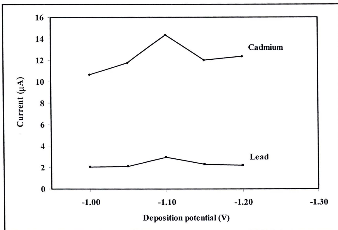
Figure 4.18 Effect of the deposition potential on the stripping peak currents for 25 \mu\text{g}\cdot\text{L}^{-1} of cadmium (II) and lead (II) ions in 0.1 M acetate buffer solutions (pH 4.5) recorded with 2.00 mol % Bi-CNT/GC electrodes by SWASV using the same experimental conditions as those in Fig. 4.15.
