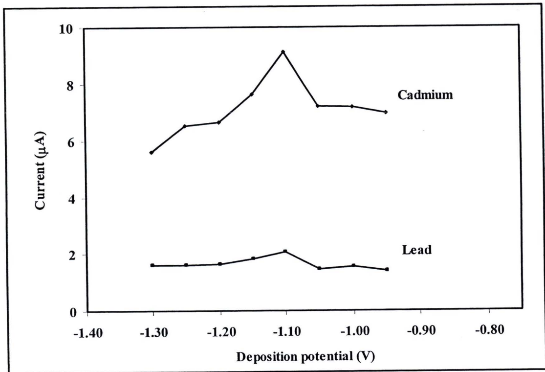
Figure 4.11 Effect of the deposition potential on the stripping peak currents for 25 \mu\text{g}\cdot\text{L}^{-1} of cadmium (II) and lead (II) ions in 0.1 M acetate buffer solutions (pH 4.5) recorded with in situ BiF/CNT/GC electrodes by SWASV using the same experimental conditions as those in Fig. 4.9.
