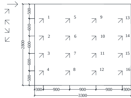
Figure 2. The number and location of measuring point of strain on No.1-1 and 2-1.
