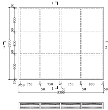
Figure 1. Construction and Size of husk mortar composite wallboard No. 1-1 and 2-1.
