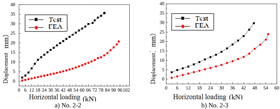
Figure 4. The load displacement curve.
