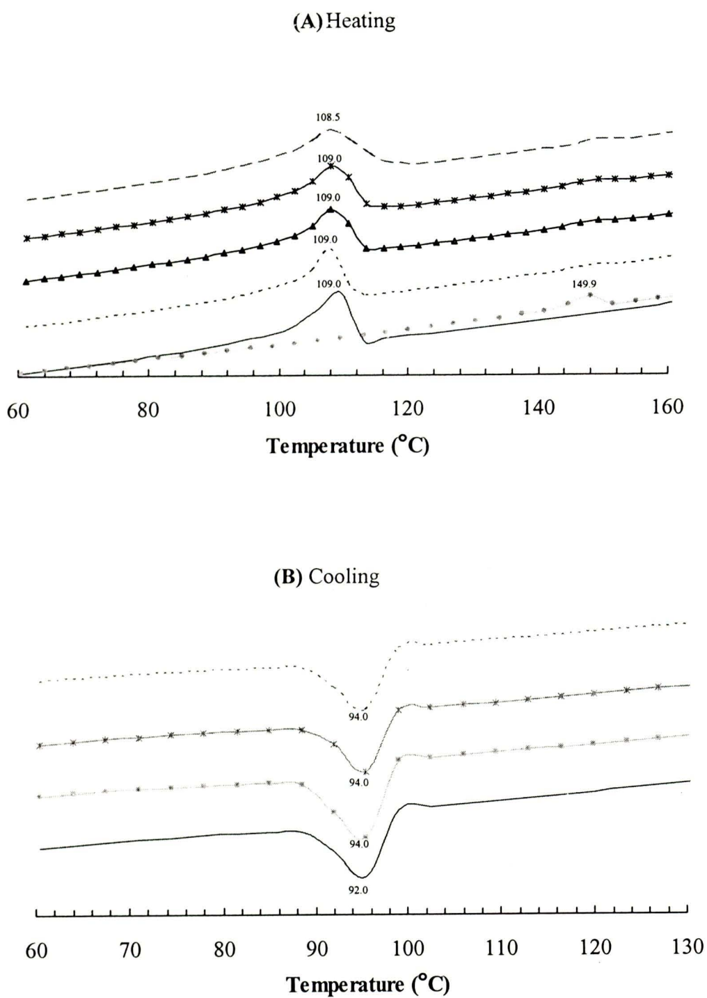
Figure 4.11 DSC thermograms of PLA, LDPE125KD and uncompatibilized LDPE125KD/PLA blends:
