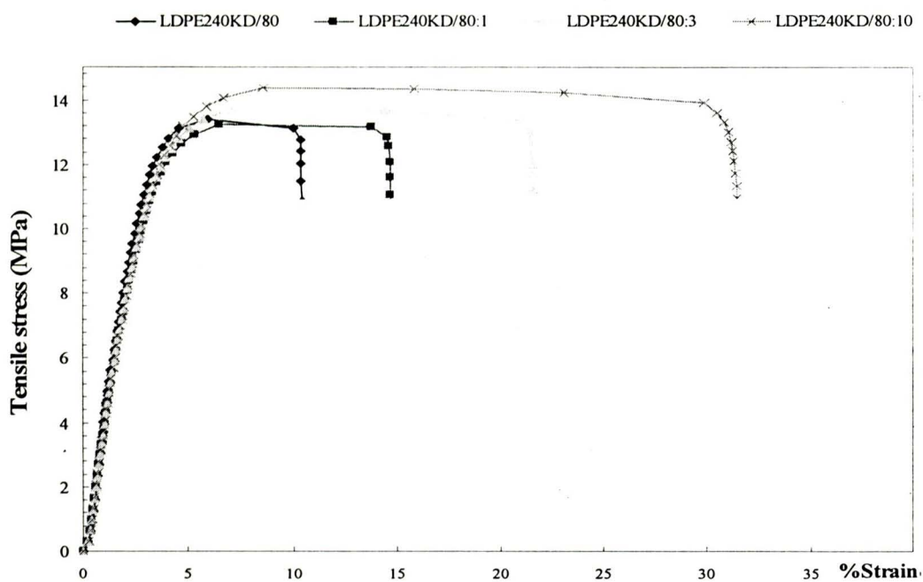
(B) The uncompatibilized and compatibilized LDPE240KD/80 blends
