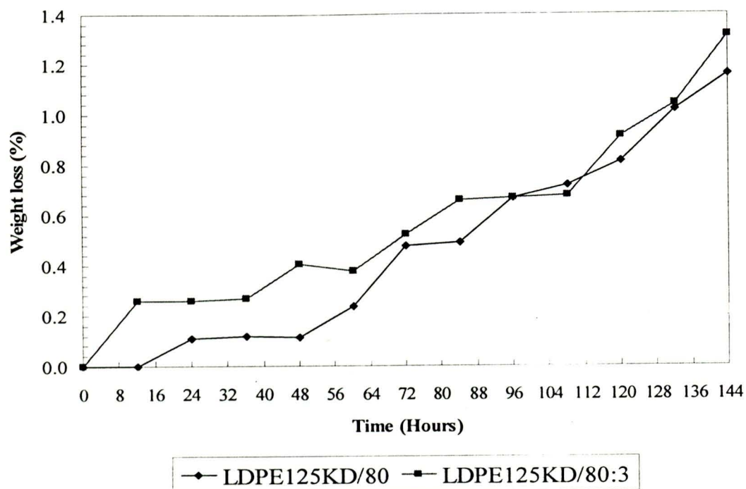
Figure 4.31 Weight loss of the uncompatibilized and compatibilized LDPE125KD/80
