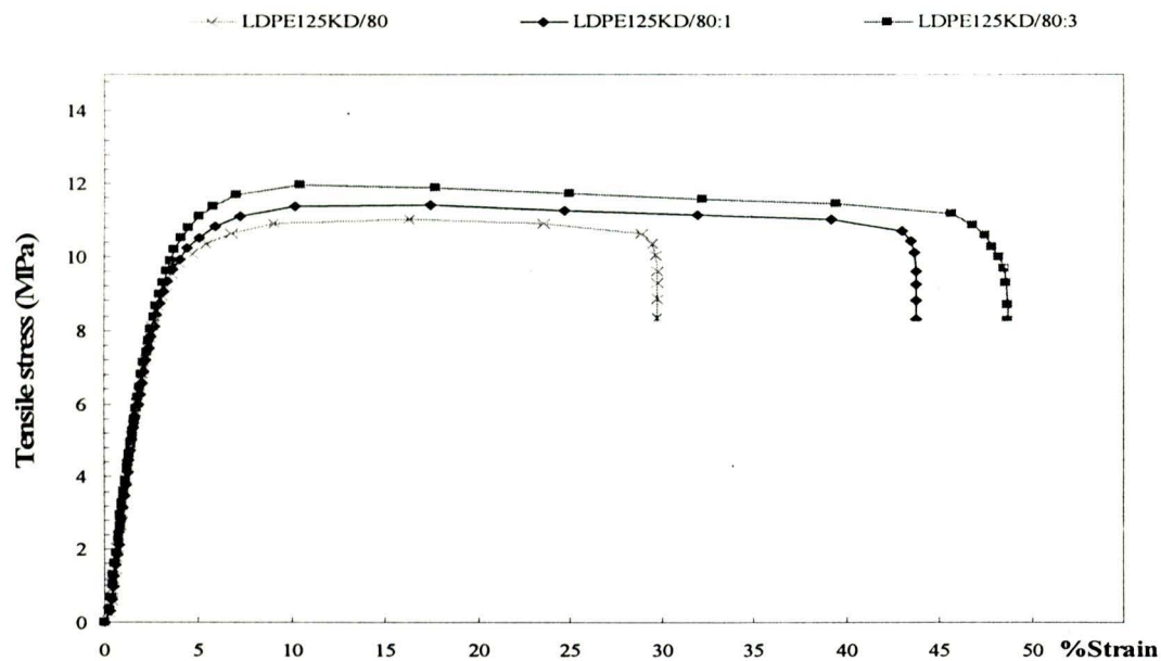
(B) The uncompatibilized and compatibilized LDPE125KD/80 blends
