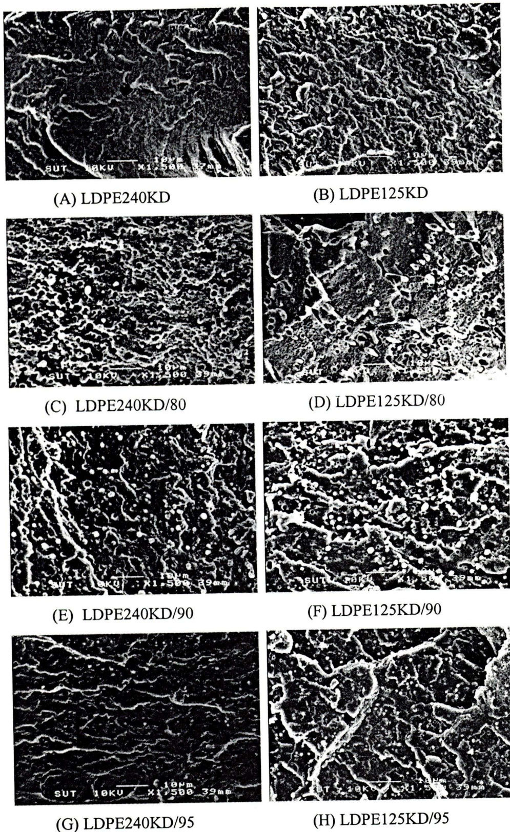
Figure 4.3 Scanning electron micrographs showing the fractured surfaces of the uncompatibilized LDPE125KD/PLA and LDPE240KD/PLA: (A) LDPE240KD; (B) LDPE125KD; (C) LDPE240KD/80; (D) LDPE125KD/80; (E) LDPE240KD/90; (F) LDPE125KD/90; (G) LDPE240KD/95; (H) LDPE125KD/95
