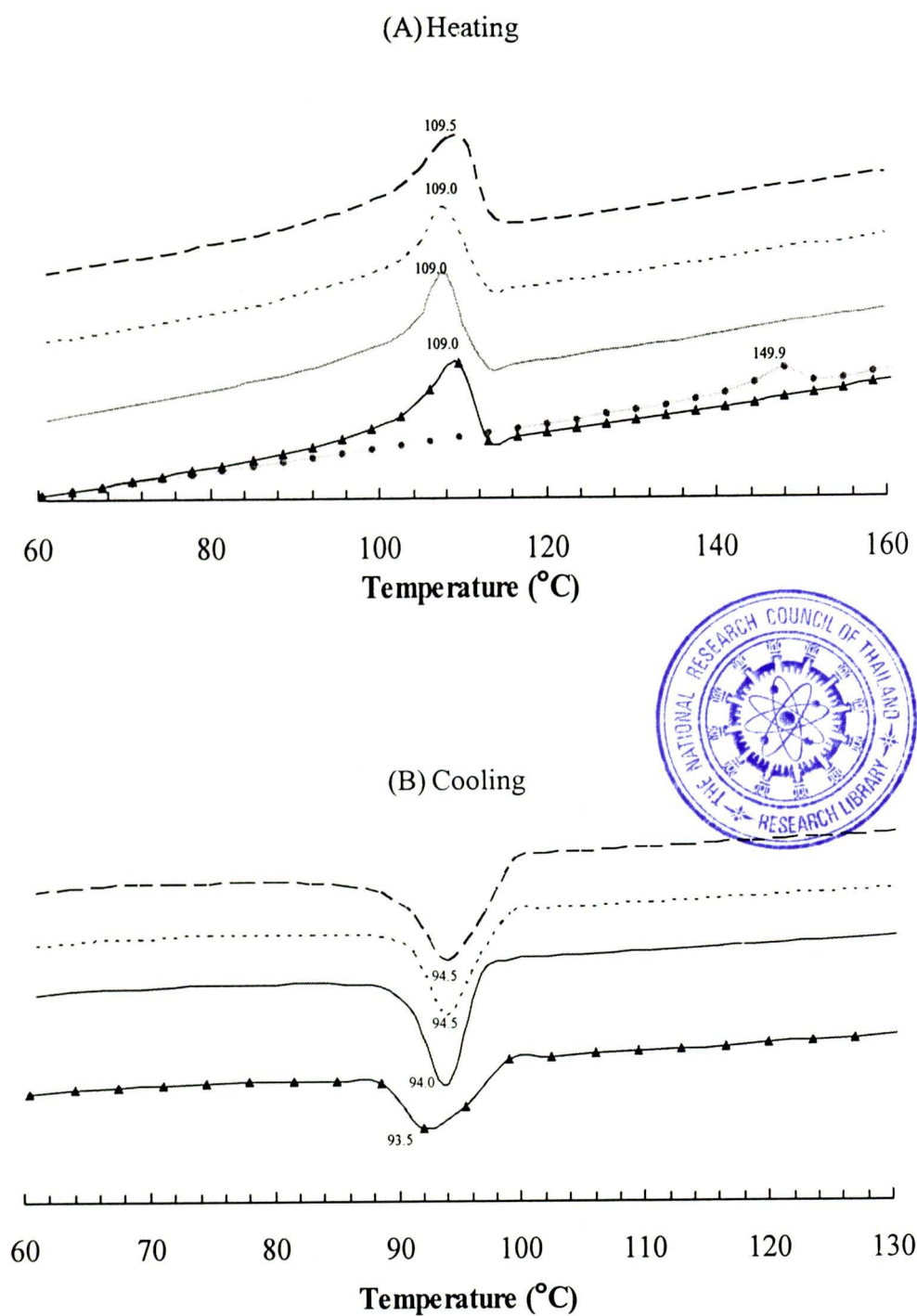
Figure 4.10 DSC thermograms of PLA, LDPE240KD, LDPE240KD/95 blends uncompatibilized and compatibilized with LLDPE-g-MA:
