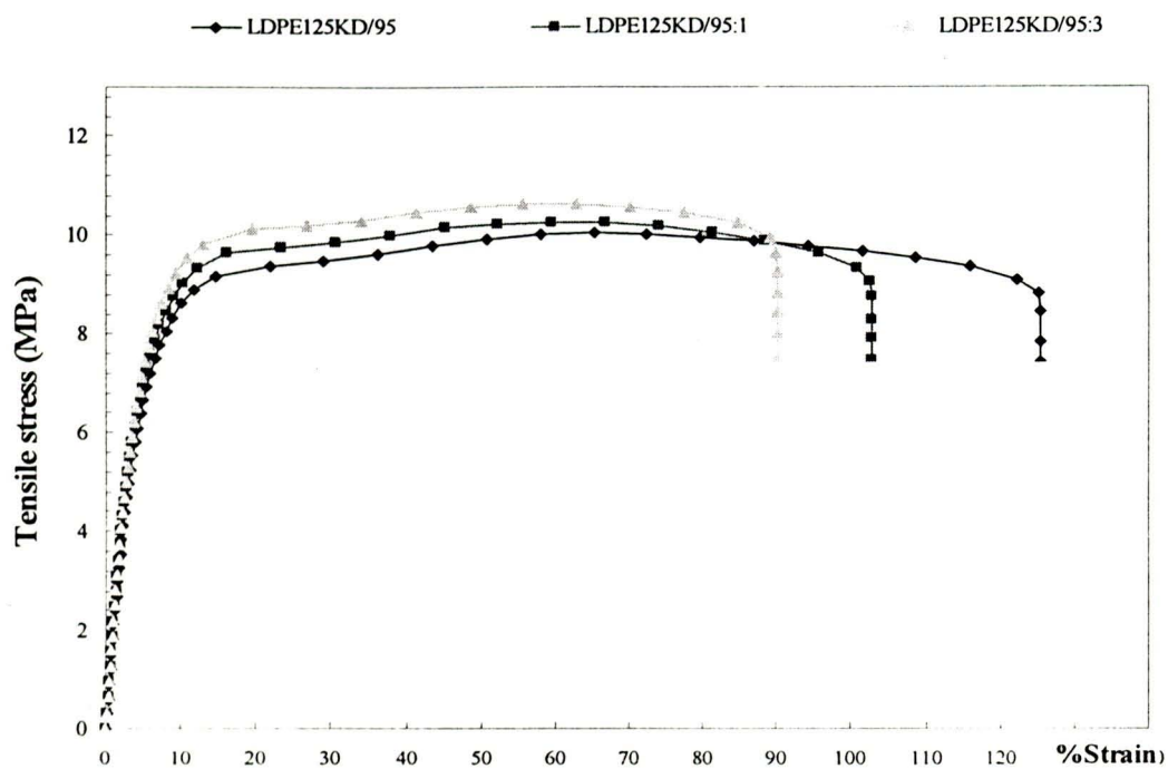
(A) The uncompatibilized and compatibilized LDPE125KD/95 blends
