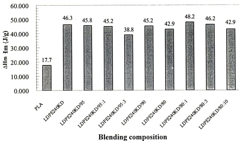
(A) LDPE240KD, PLA and their blends
