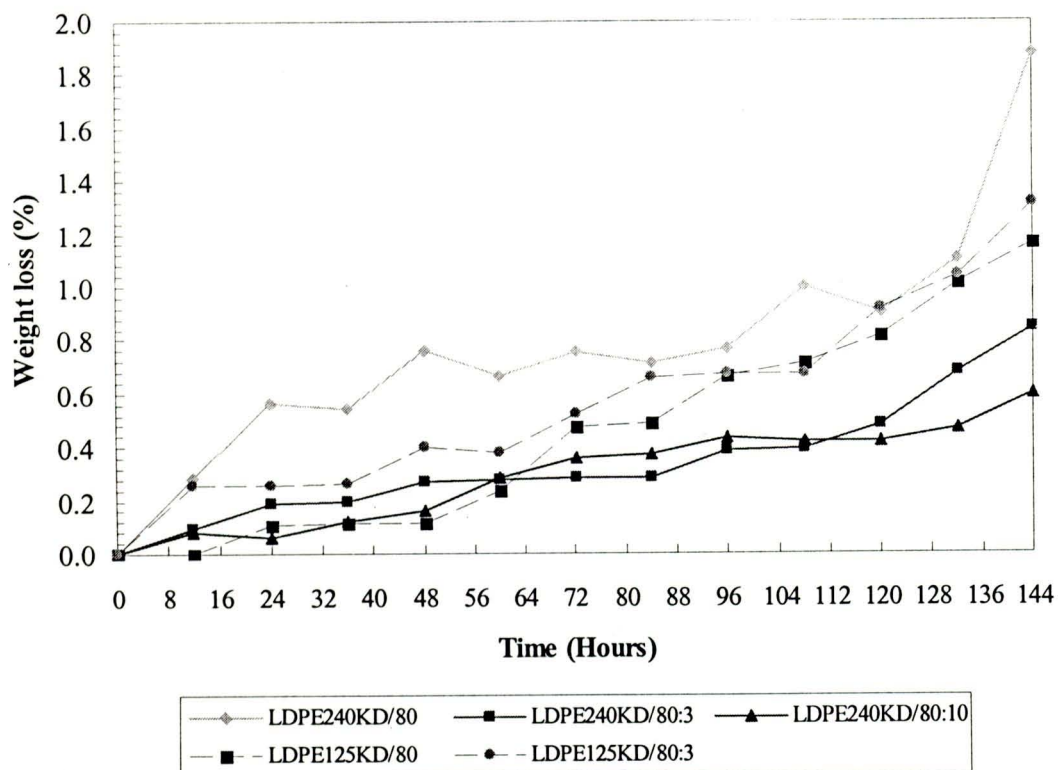
Figure 4.32 Comparison of weight loss between LDPE240KD/80 and LDPE125KD/80
