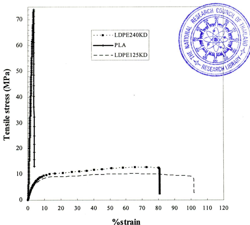
Figure 4.22 Tensile strength of PLA, LDPE125KD and LDPE240KD
