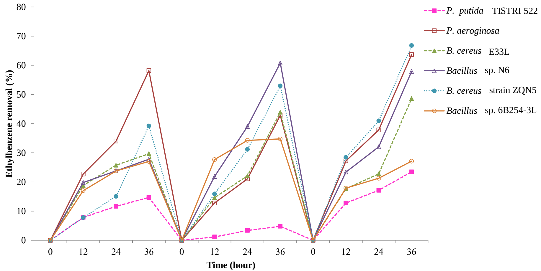
Figure 4.6 Percentage of ethylbenzene removal by only microorganism-associated leaf of Z. zamiffolia in 3 cycles
