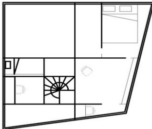
2F plan
