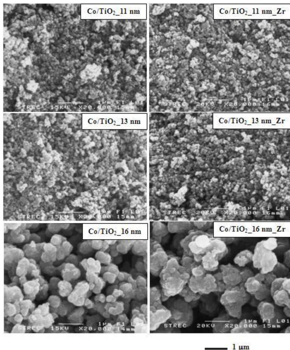
Fig. 2. SEM micrographs of Co catalysts with and without Zr-modified different crystallite sizes of \text{TiO}_2 supports.
