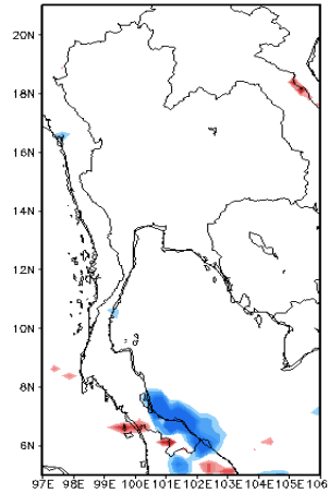
Diff Exp05–Obv on 15hr 23/Nov/2011
