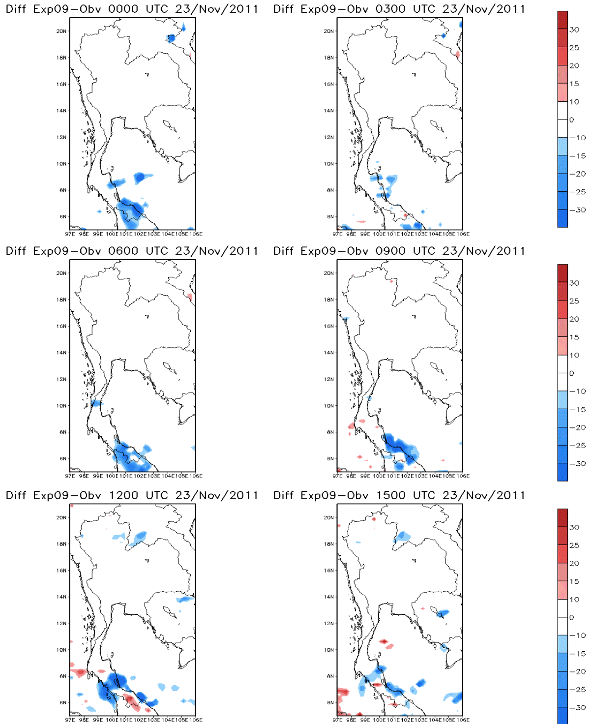
Figure I01 The different of rainfall distribution pattern between observation data of Exp09 during 0000 UTC to 1500 UTC 23 November 2011
