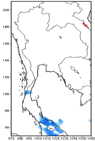
Diff Exp05–Obv on 12hr 23/Nov/2011
