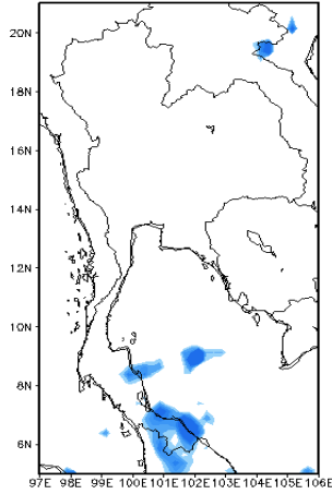
Diff Exp05–Obv on 06hr 23/Nov/2011
