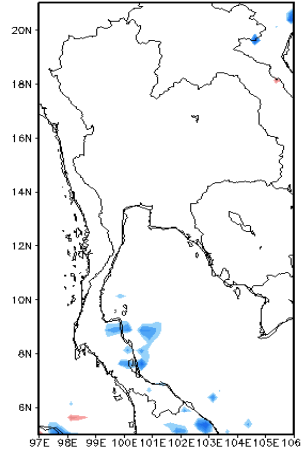
Diff Exp05–Obv on 09hr 23/Nov/2011
