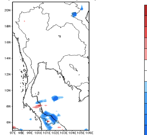
Figure I02 The different of rainfall distribution pattern between observation data of Exp09 during 0900 UTC to 1500 UTC 23 November 2011
