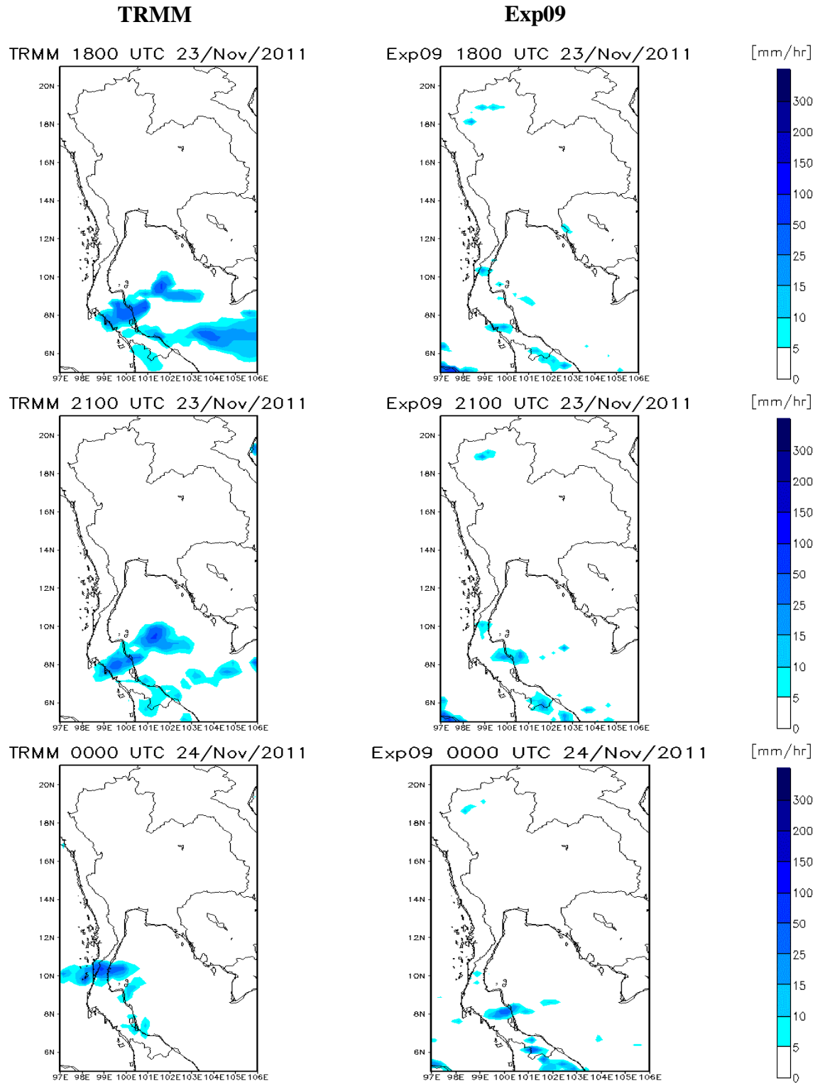
Figure H03 The comparison of rainfall distribution pattern between observation data of Exp09 during 1800 UTC 23 November 2011 to 0000 UTC 24 November 2011
