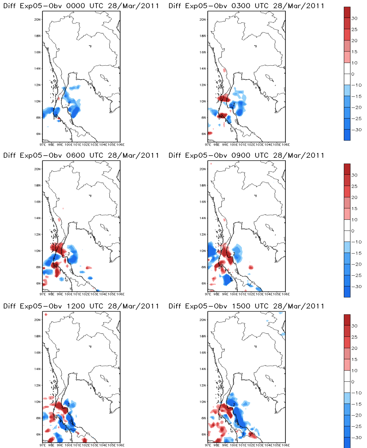
Figure E01 The different of rainfall distribution pattern between observation data of Exp05 during 0000 UTC to 1500 UTC 28 March 2011
