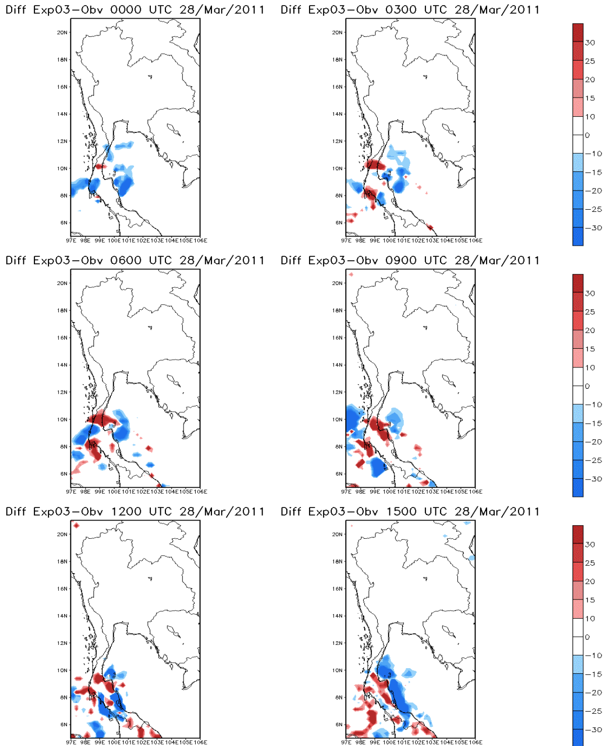
Figure E03 The different of rainfall distribution pattern between observation data of Exp03 during 0000 UTC to 1500 UTC 28 March 2011
