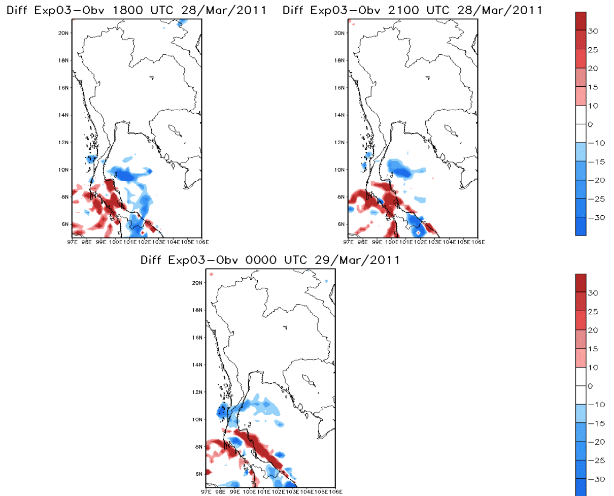
Figure E04 The different of rainfall distribution pattern between observation data of Exp03 during 1800 UTC 28 March 2011 to 0000 UTC 29 March 2011
