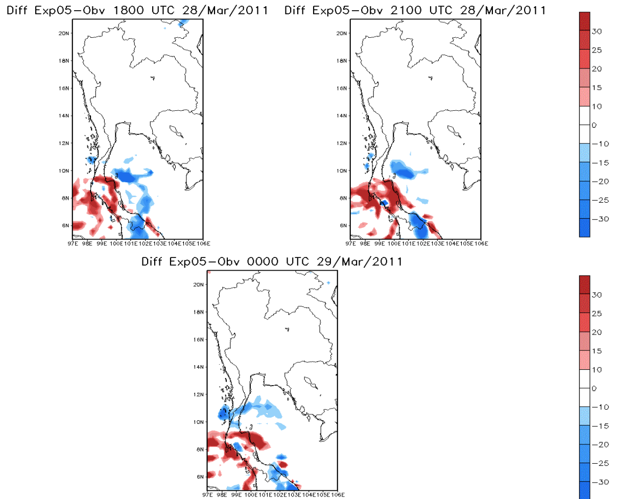
Figure E02 The different of rainfall distribution pattern between observation data of Exp05 during 1800 UTC 28 March 2011 to 0000 UTC 29 March 2011
