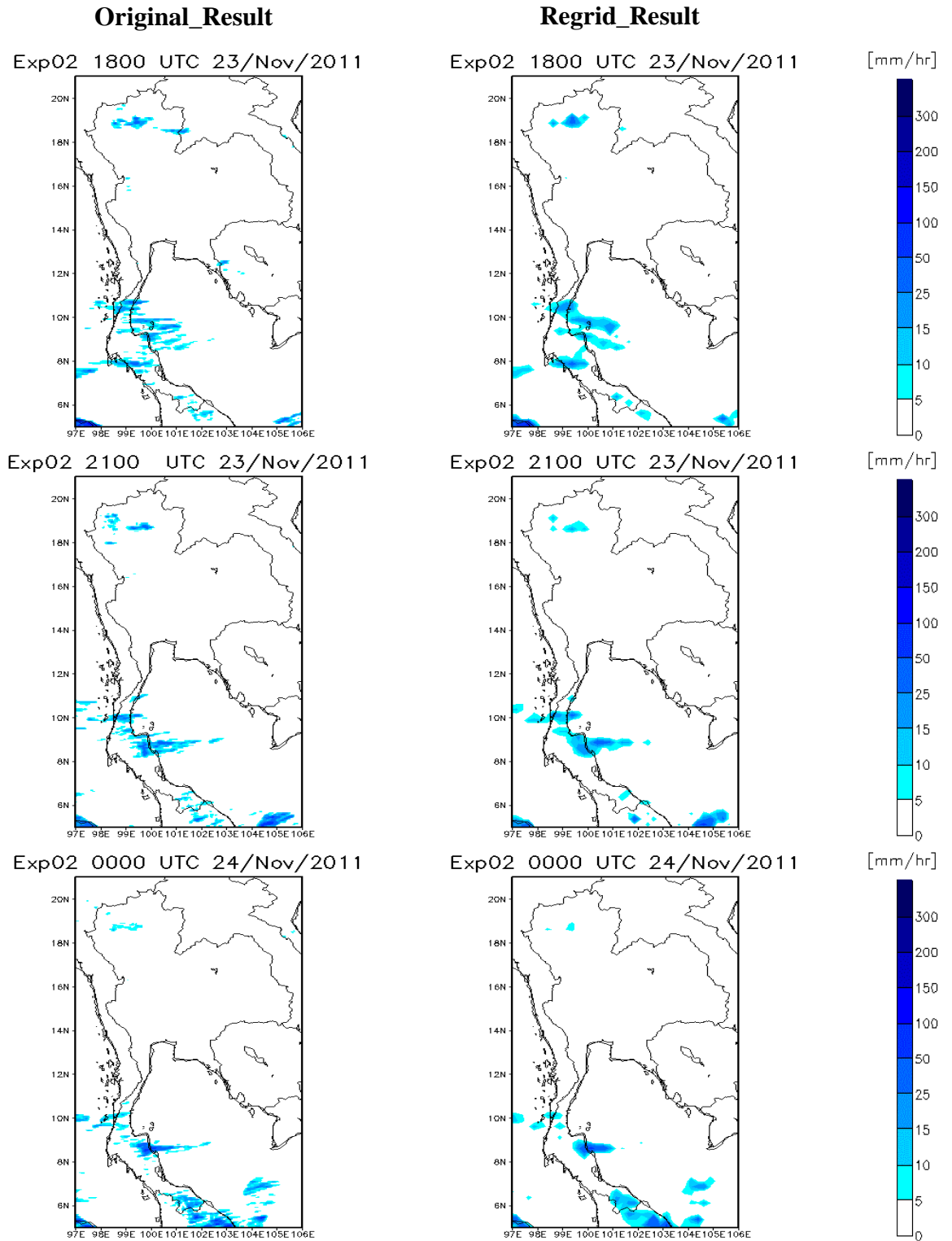
Figure C06. The comparison of rainfall distribution pattern between the original results and re-gridding results during 1800 UTC 23 November 2011 to 0000 UTC 24 November 2011 of Exp02
