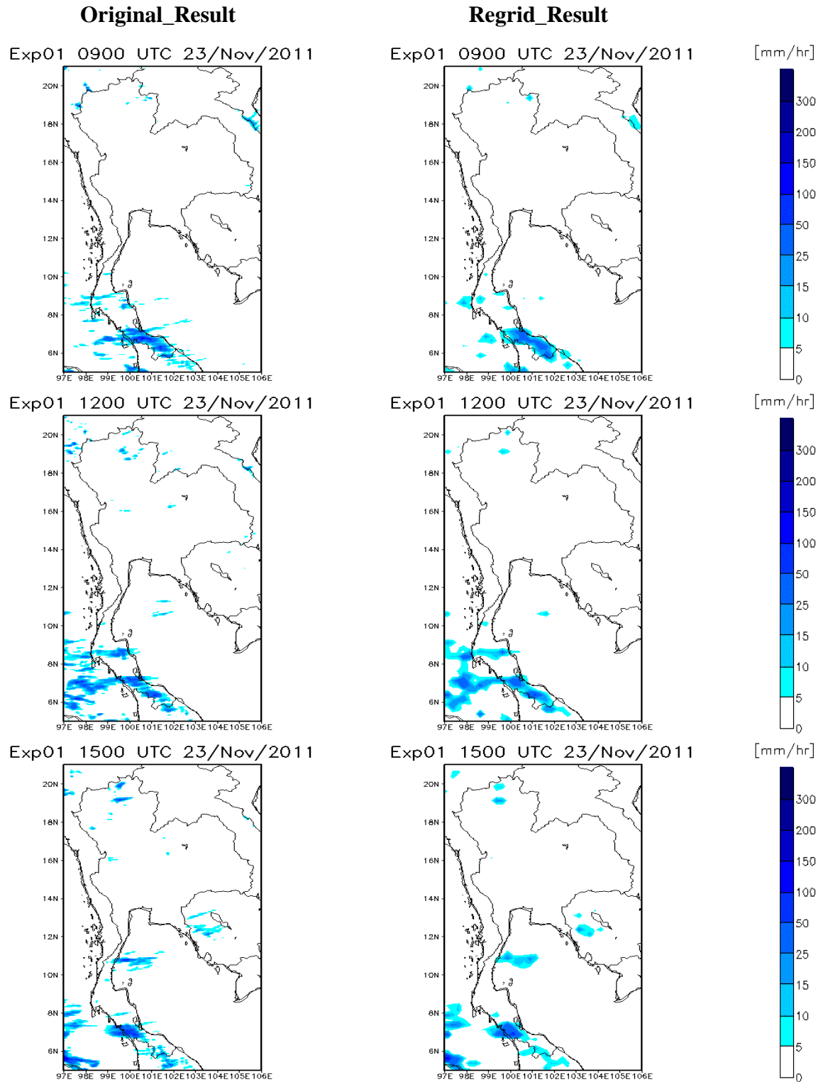
Figure C02. The comparison of rainfall distribution pattern between the original results and re-gridding results during 0900 UTC to 1500 UTC 23 November 2011 of Exp01
