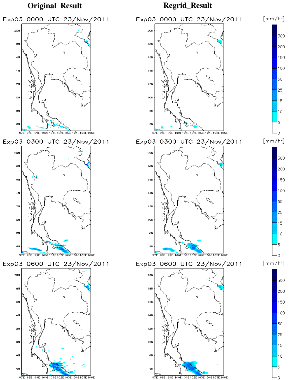
Figure C07. The comparison of rainfall distribution pattern between the original results and re-gridding results during 0000 UTC to 0600 UTC 23 November 2011 of Exp03
