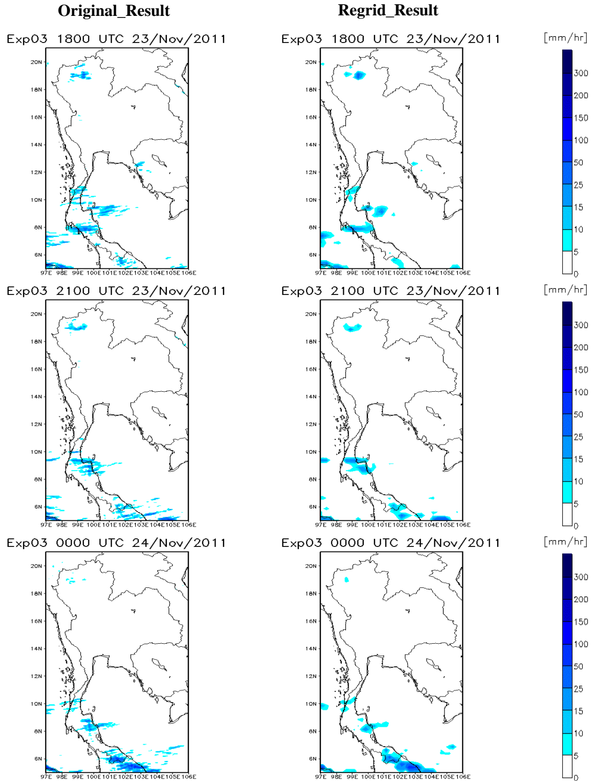
Figure C09. The comparison of rainfall distribution pattern between the original results and re-gridding results during 1800 UTC 23 November 2011 to 0000 UTC 24 November 2011 of Exp03
