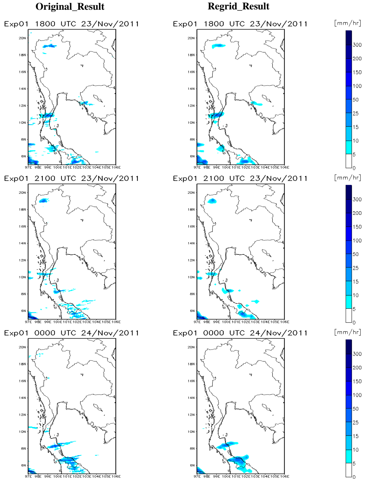
Figure C03. The comparison of rainfall distribution pattern between the original results and re-gridding results during 1800 UTC 23 November 2011 to 0000 UTC 24 November 2011 of Exp01
