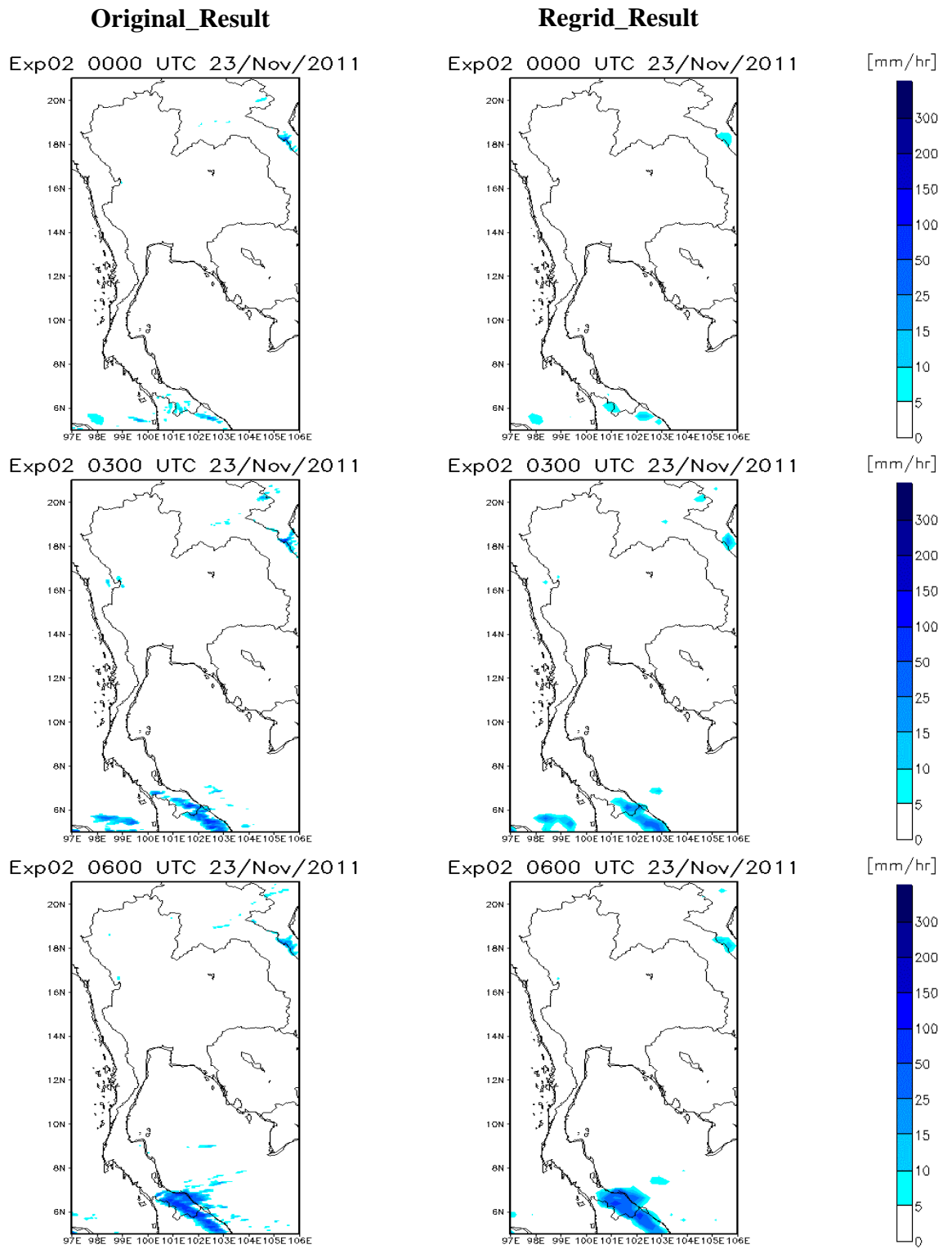
Figure C04. The comparison of rainfall distribution pattern between the original results and re-gridding results during 0000 UTC to 0600 UTC 23 November 2011 of Exp02
