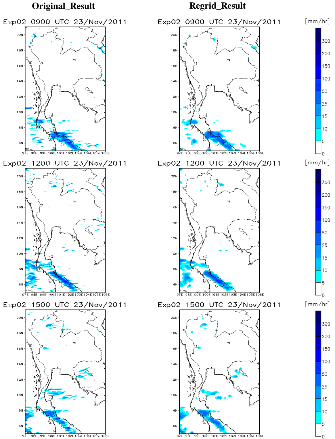
Figure C05. The comparison of rainfall distribution pattern between the original results and re-gridding results during 0900 UTC to 1500 UTC 23 November 2011 of Exp02
