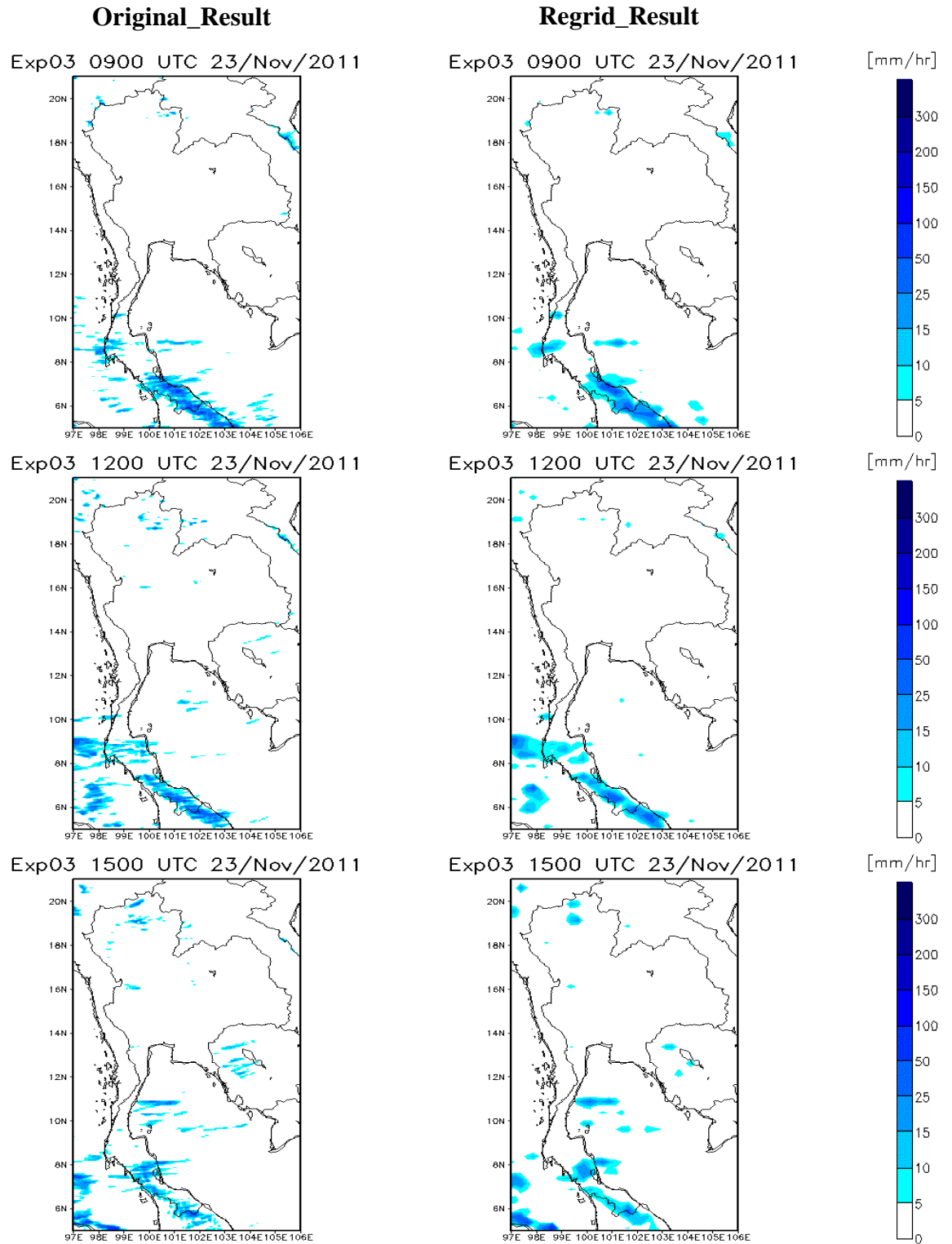
Figure C08. The comparison of rainfall distribution pattern between the original results and re-gridding results during 0900 UTC to 1500 UTC 23 November 2011 of Exp03
