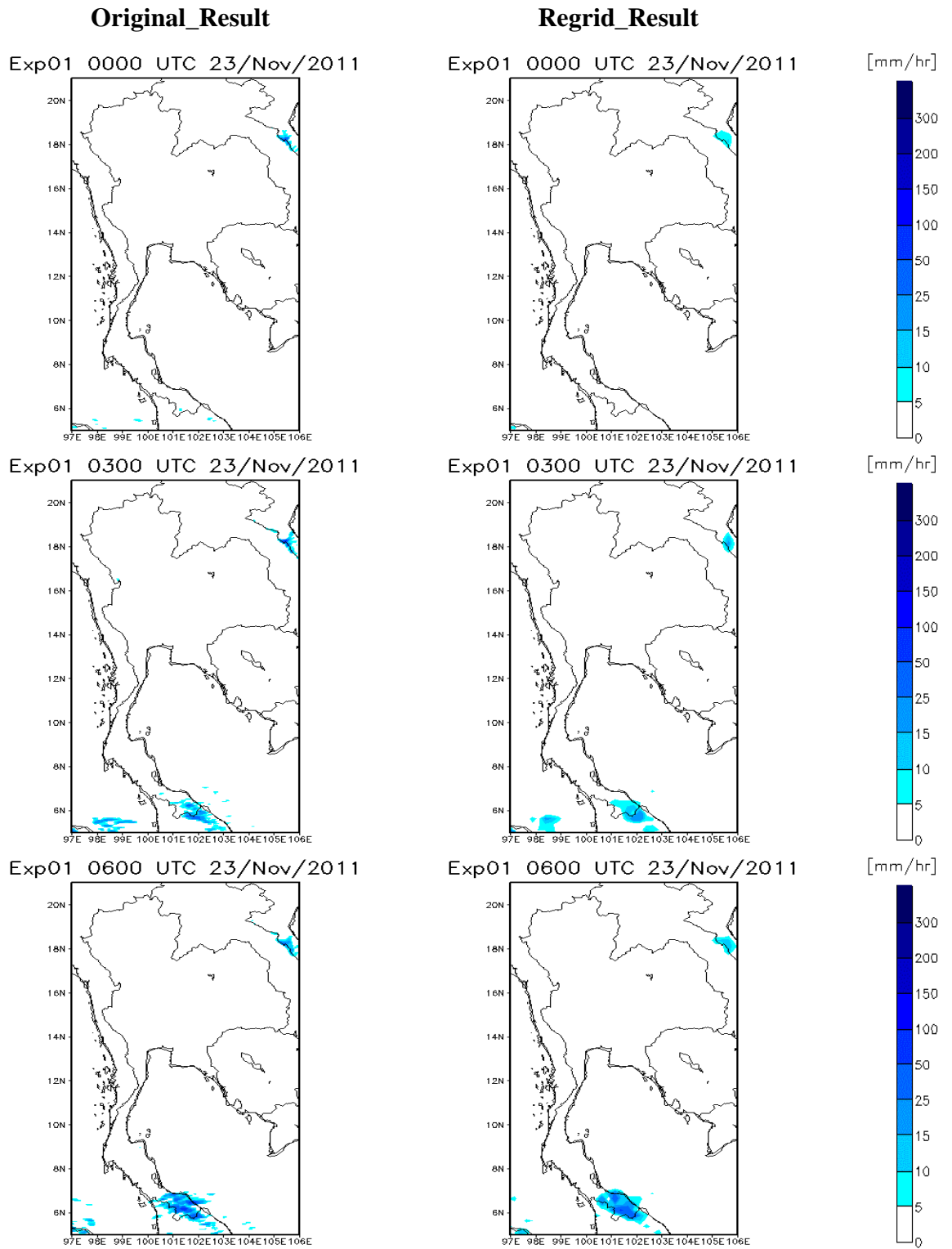
Figure C01. The comparison of rainfall distribution pattern between the original results and re-gridding results during 0000 UTC to 0600 UTC 23 November 2011 of Exp01
