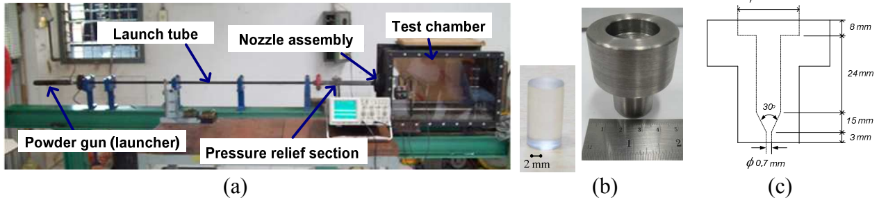
Figure 1 (a) Horizontal Single-Stage Powder Gun, (b) projectile, and (c) Nozzle geometry
