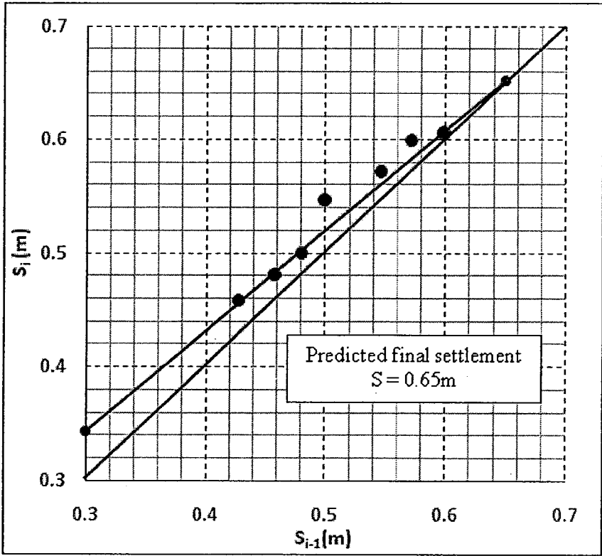
Asaoka’s Plot
