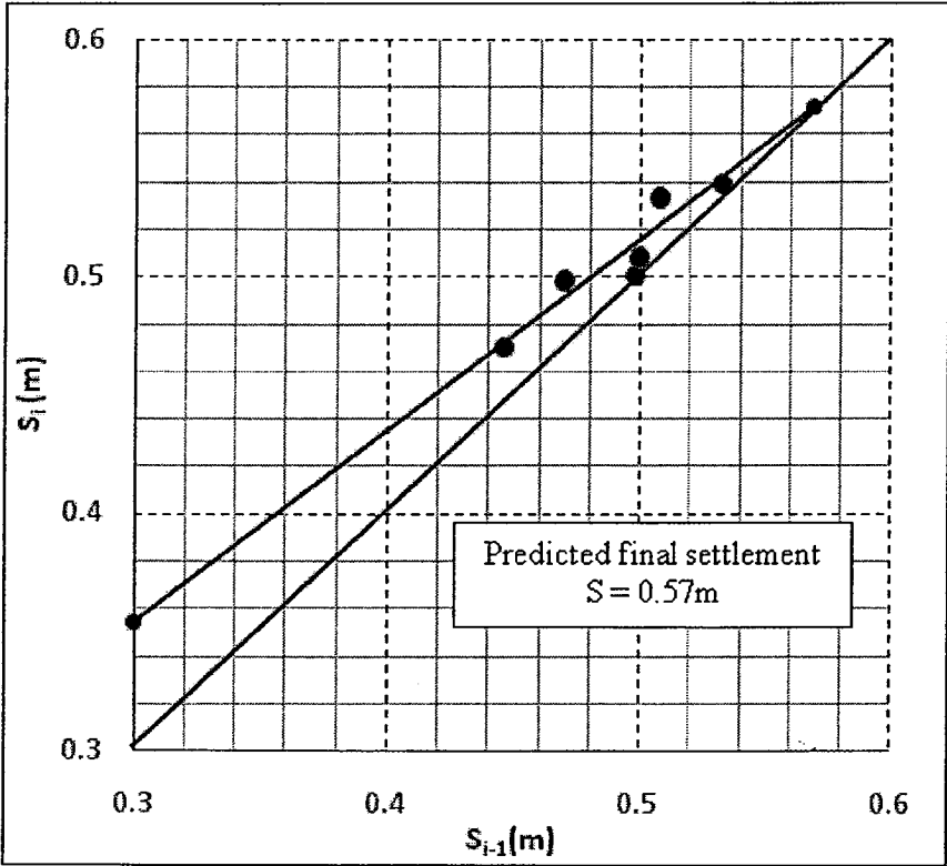
Asaoka's Plot
