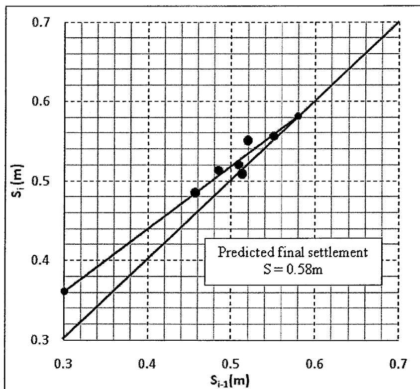
Asaoka's Plot
