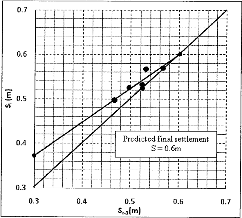
Asaoka's Plot
