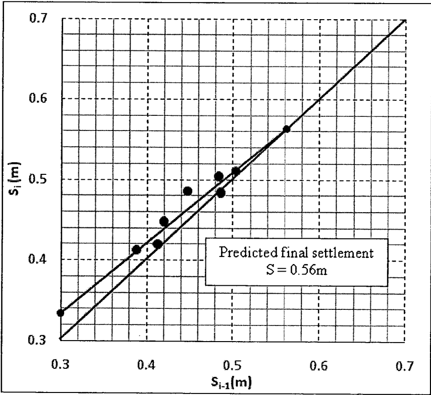
Asaoka’s Plot
