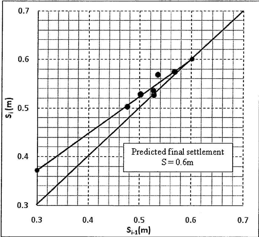
Asaoka's Plot
