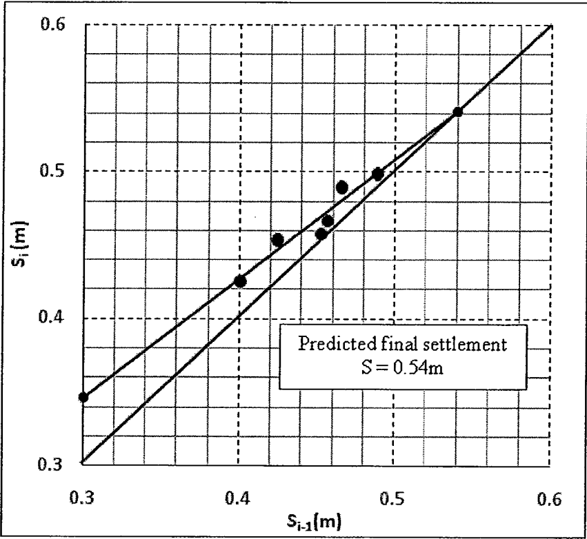
Asaoka's Plot
