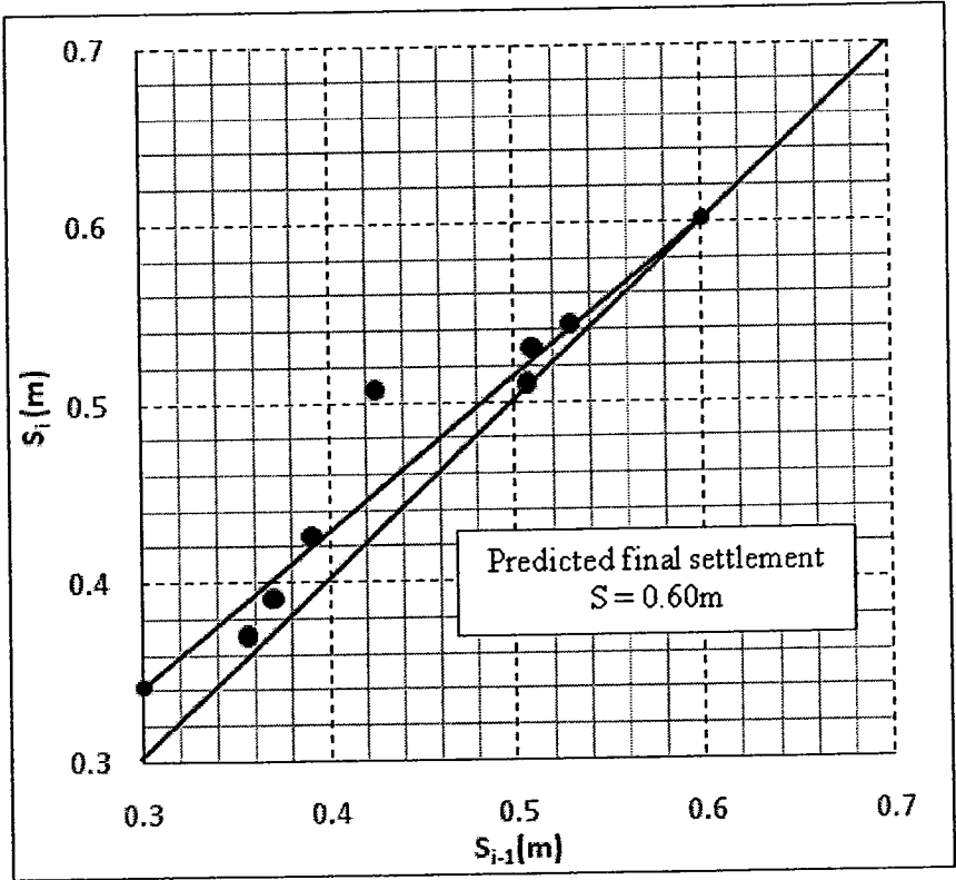
Asaoka’s Plot
